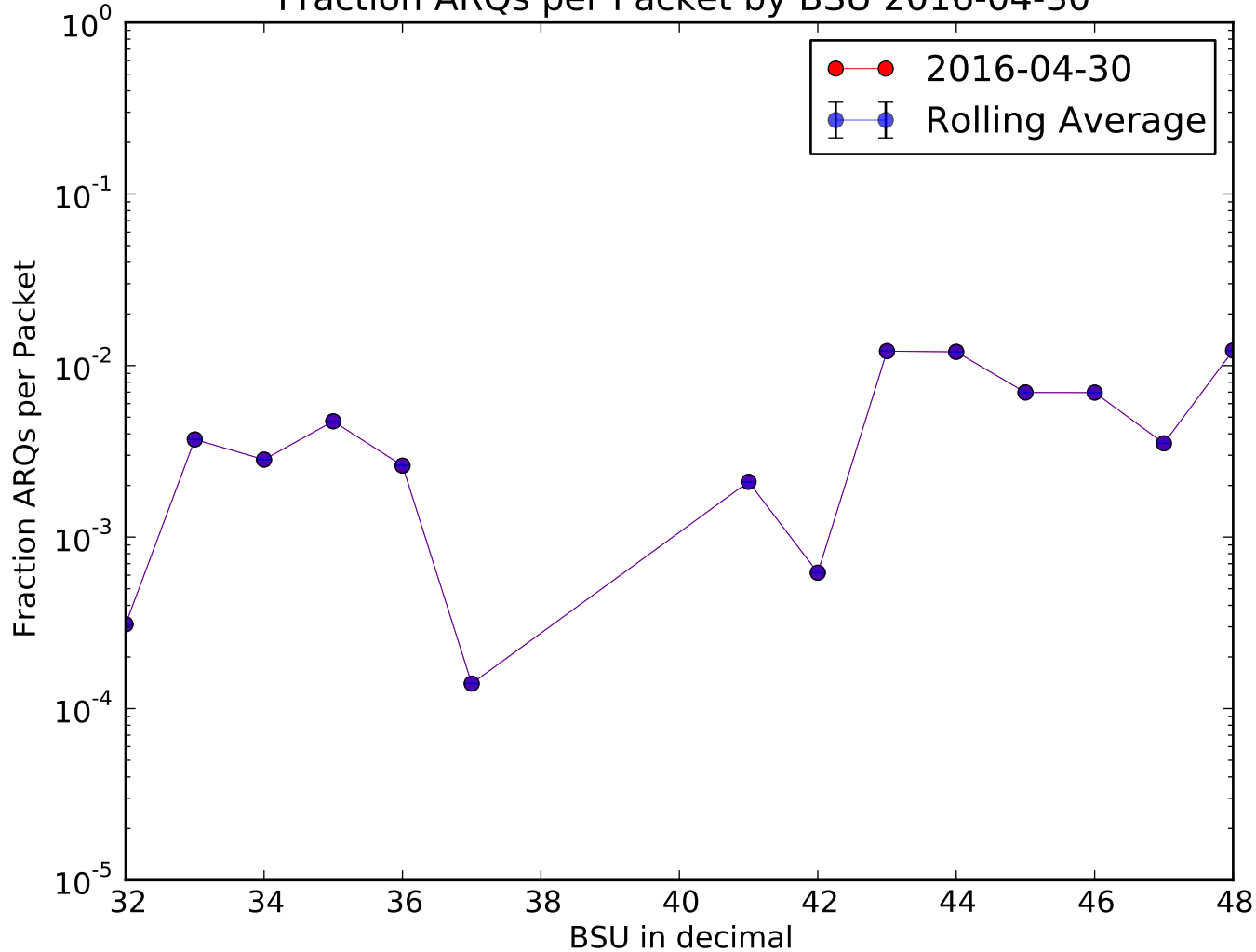
Fraction ARQs per Packet by BSU 2016-04-30
