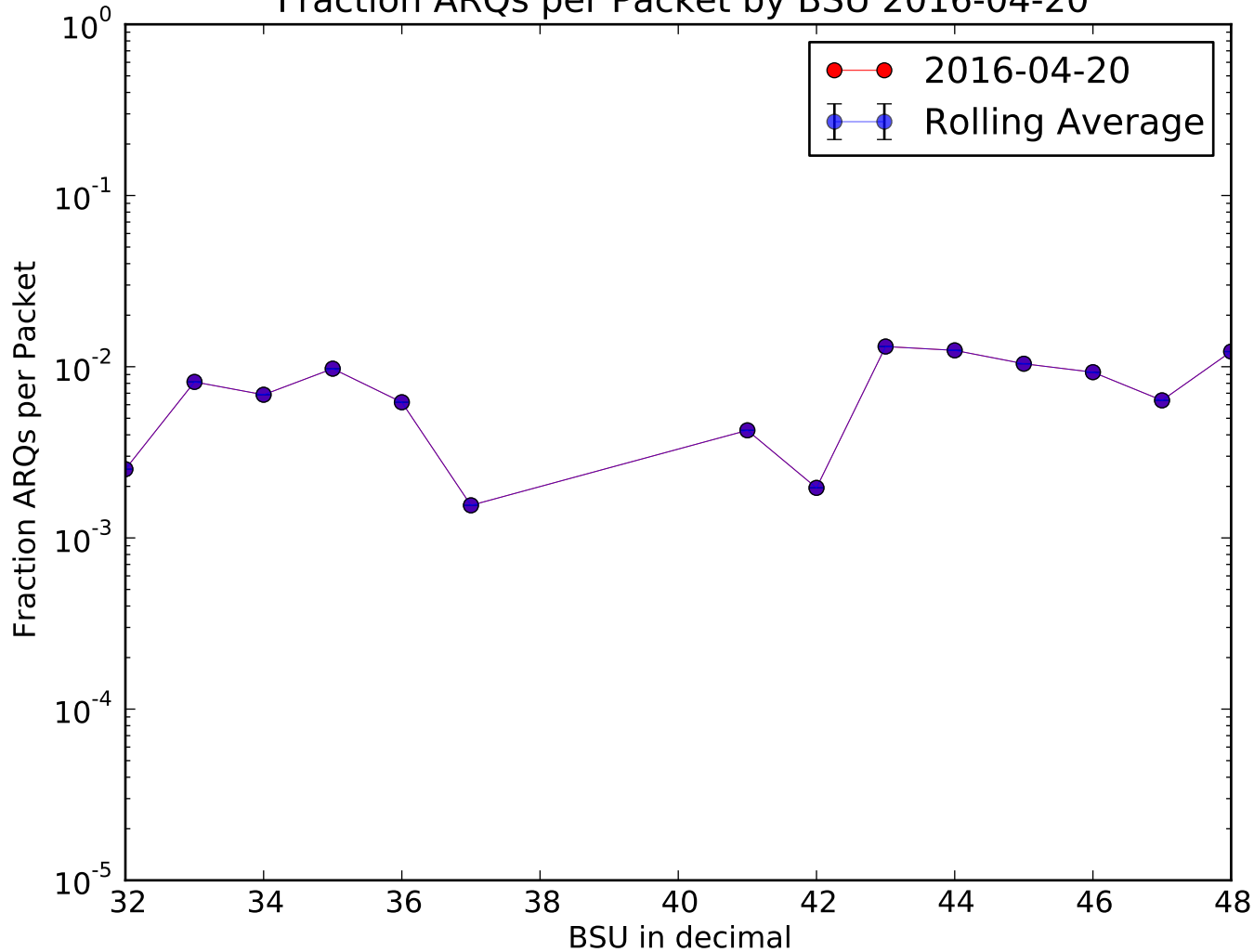
Fraction ARQs per Packet by BSU 2016-04-20
