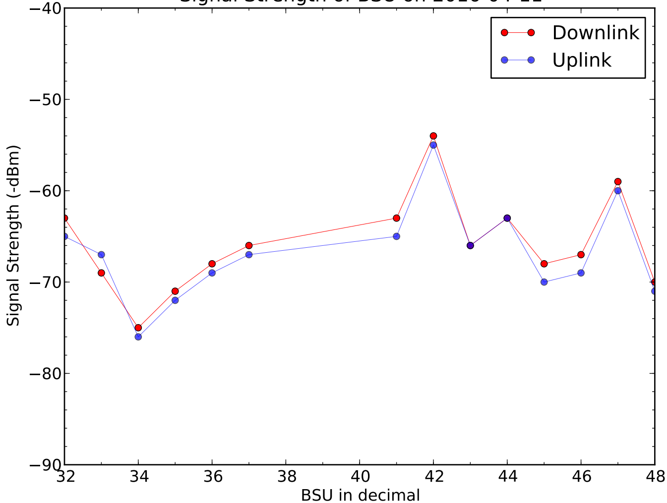
Signal Strength of BSU on 2016-04-11
