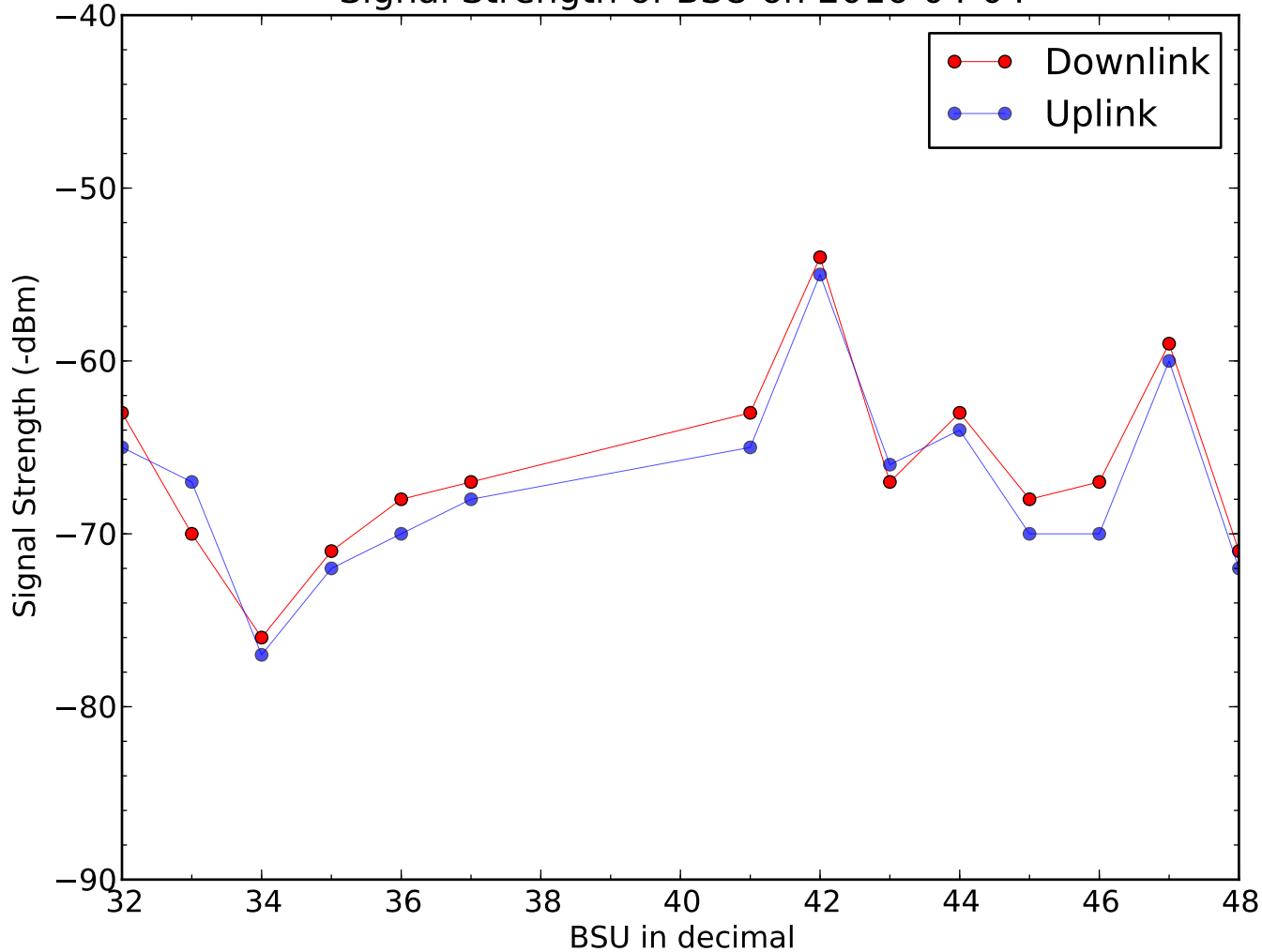
Signal Strength of BSU on 2016-04-04
