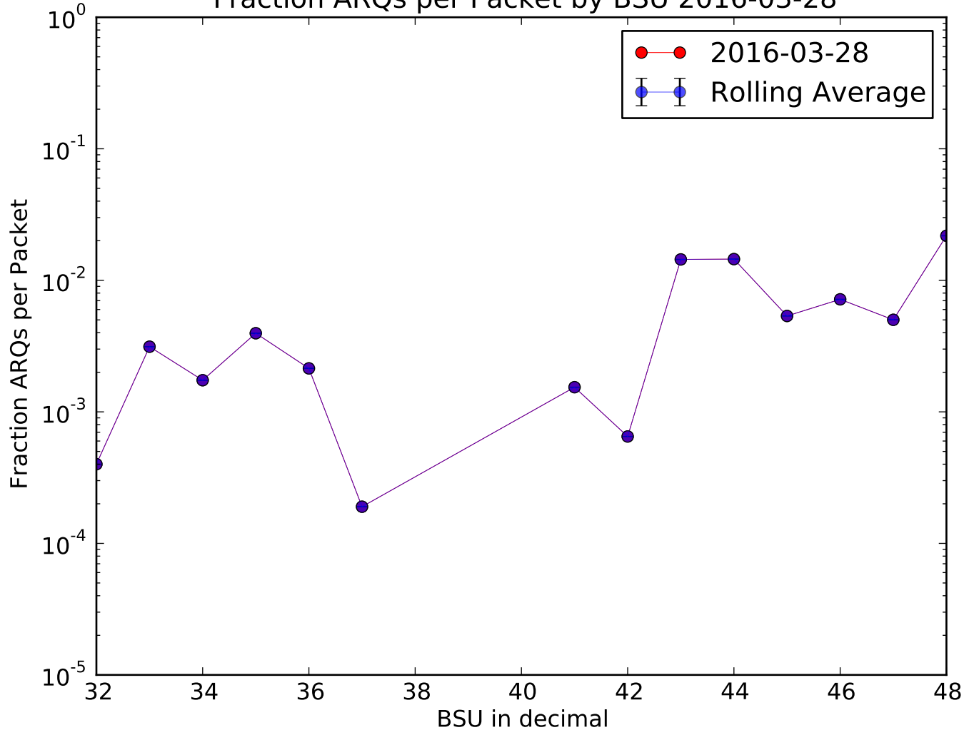
Fraction ARQs per Packet by BSU 2016-03-28
