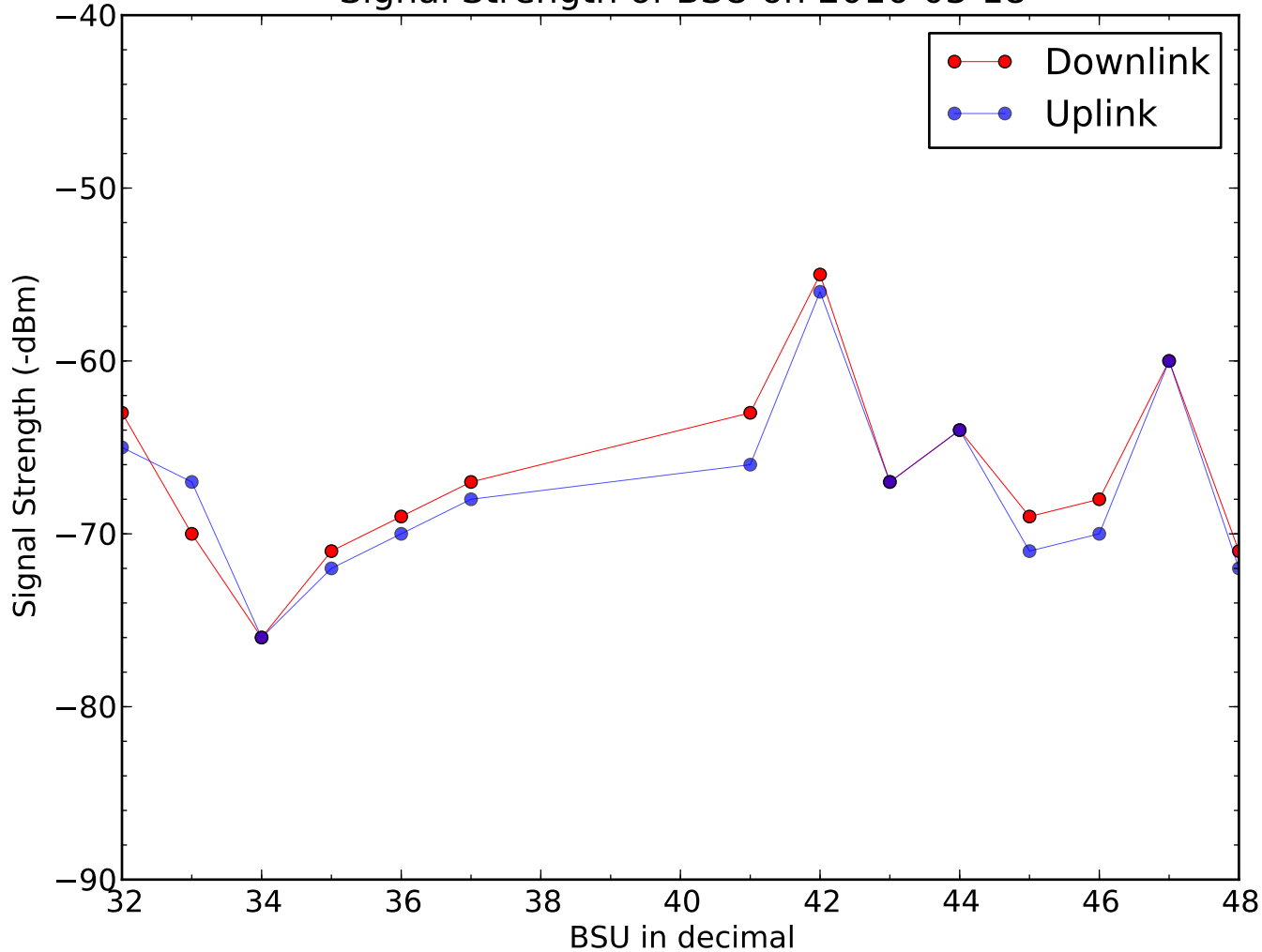
Signal Strength of BSU on 2016-03-18
