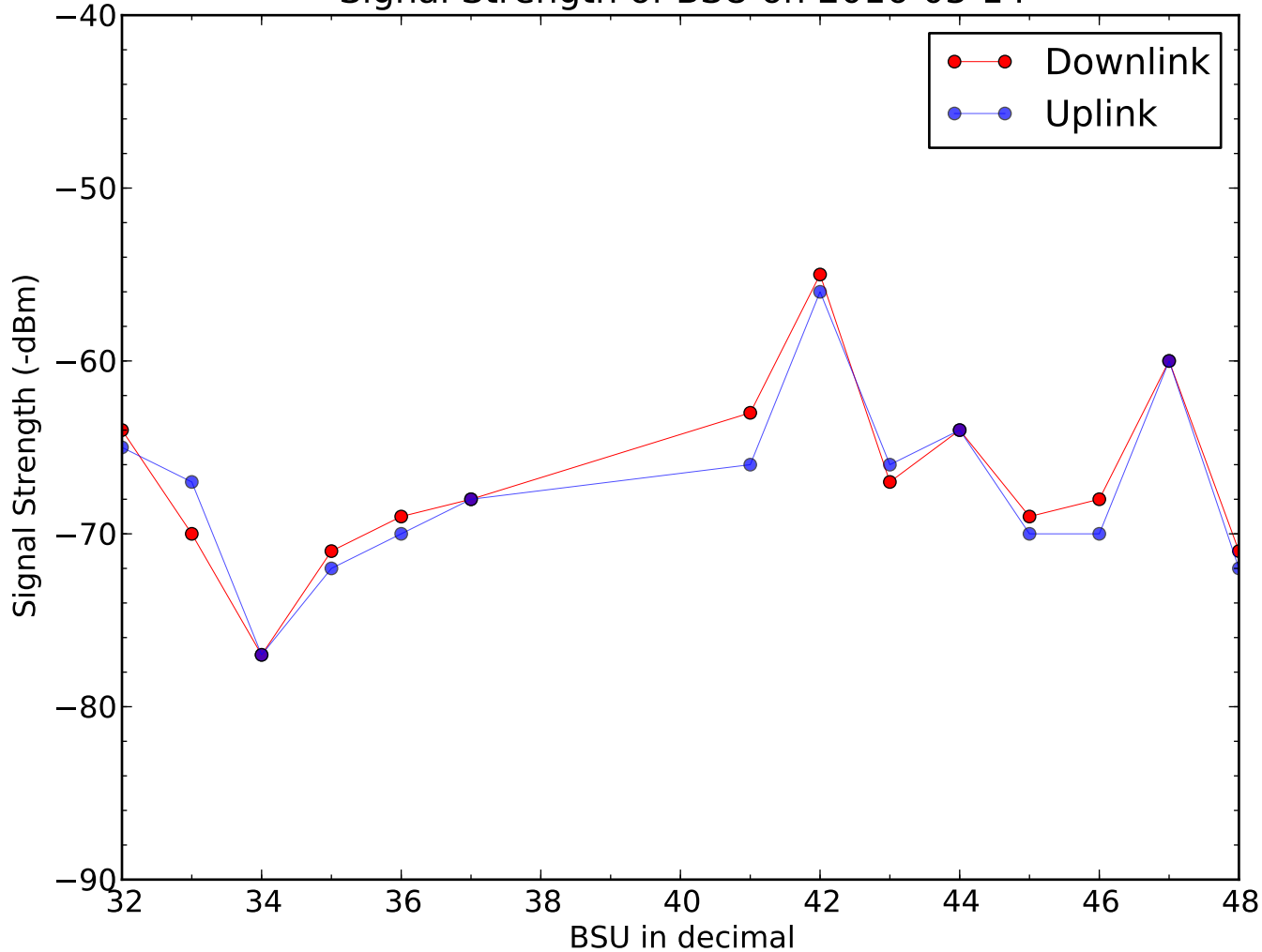
Signal Strength of BSU on 2016-03-14
