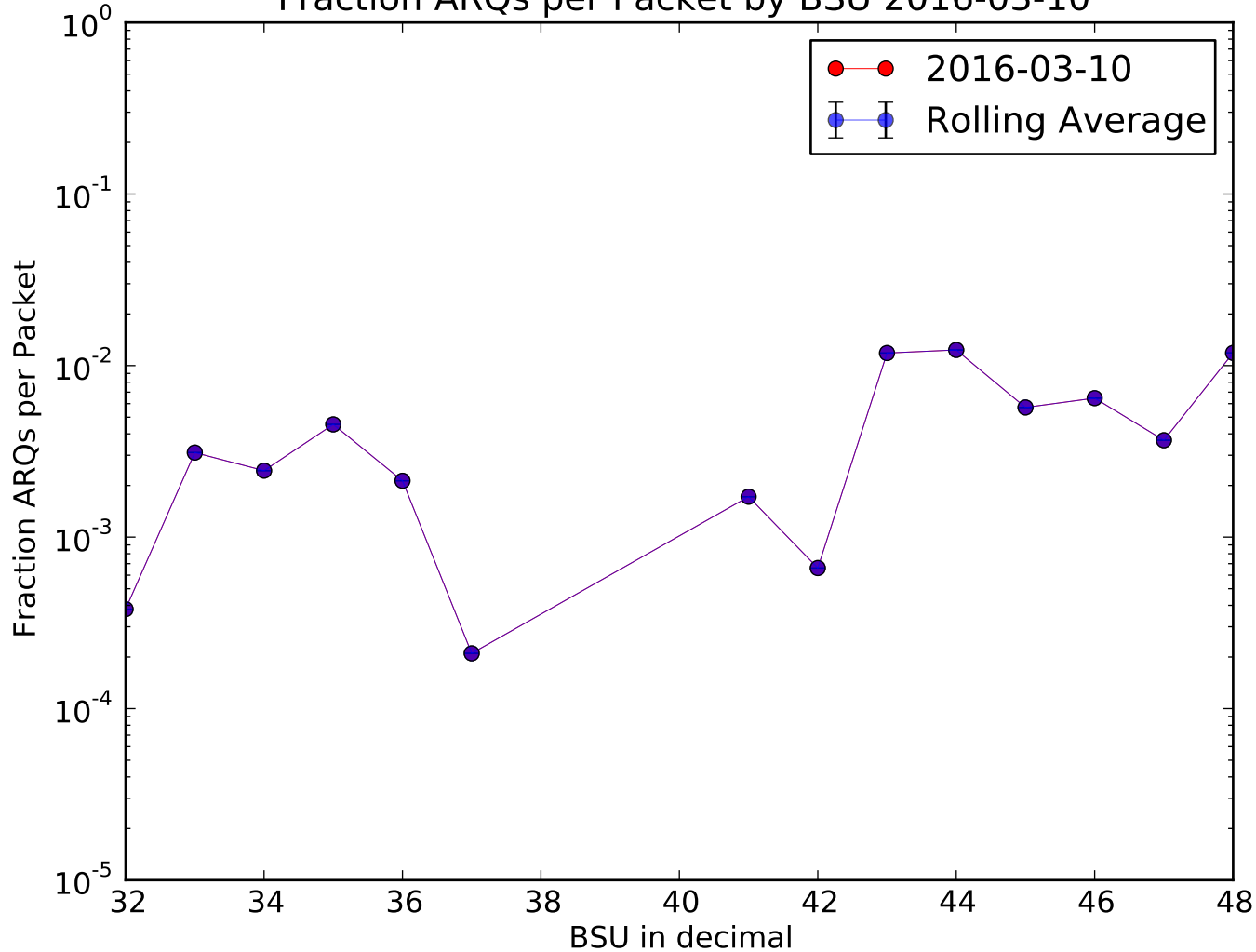
Fraction ARQs per Packet by BSU 2016-03-10
