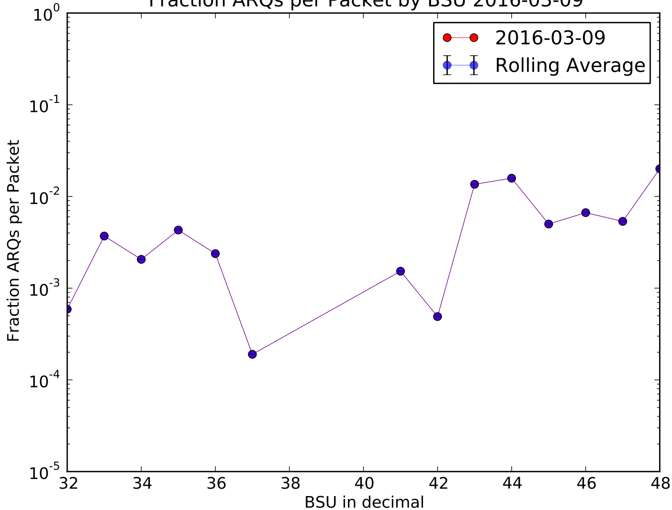
Fraction ARQs per Packet by BSU 2016-03-09
