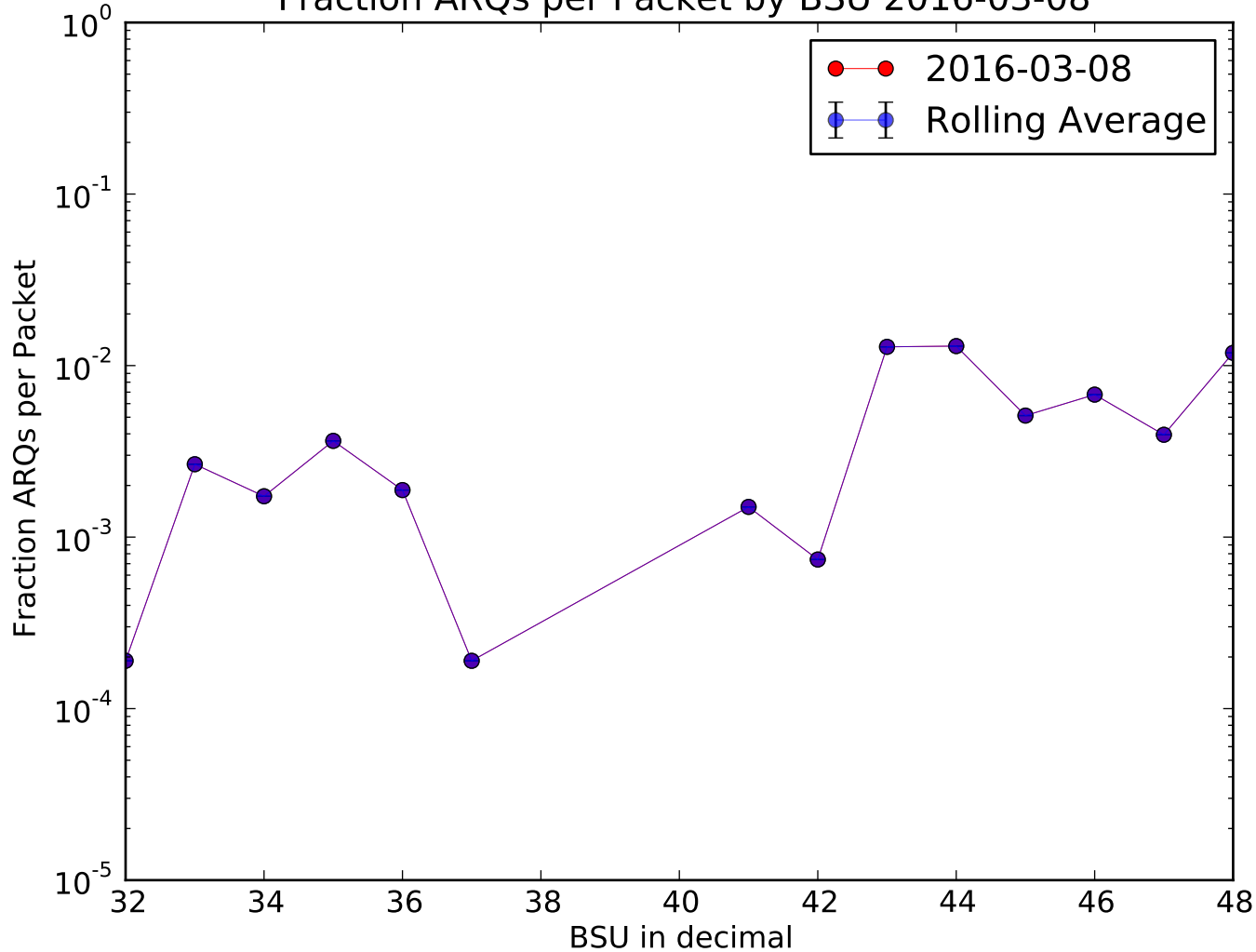
Fraction ARQs per Packet by BSU 2016-03-08
