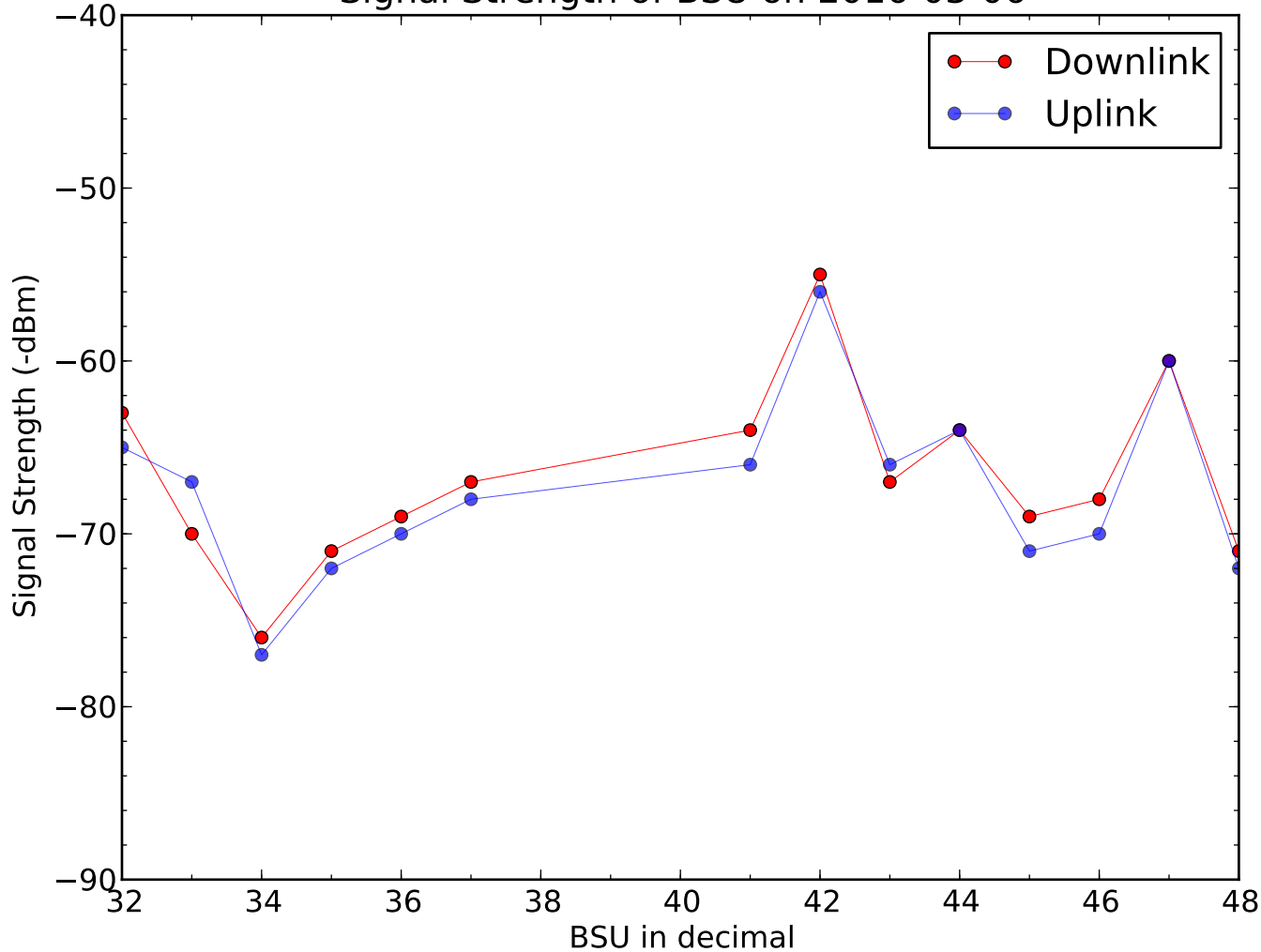
Signal Strength of BSU on 2016-03-06
