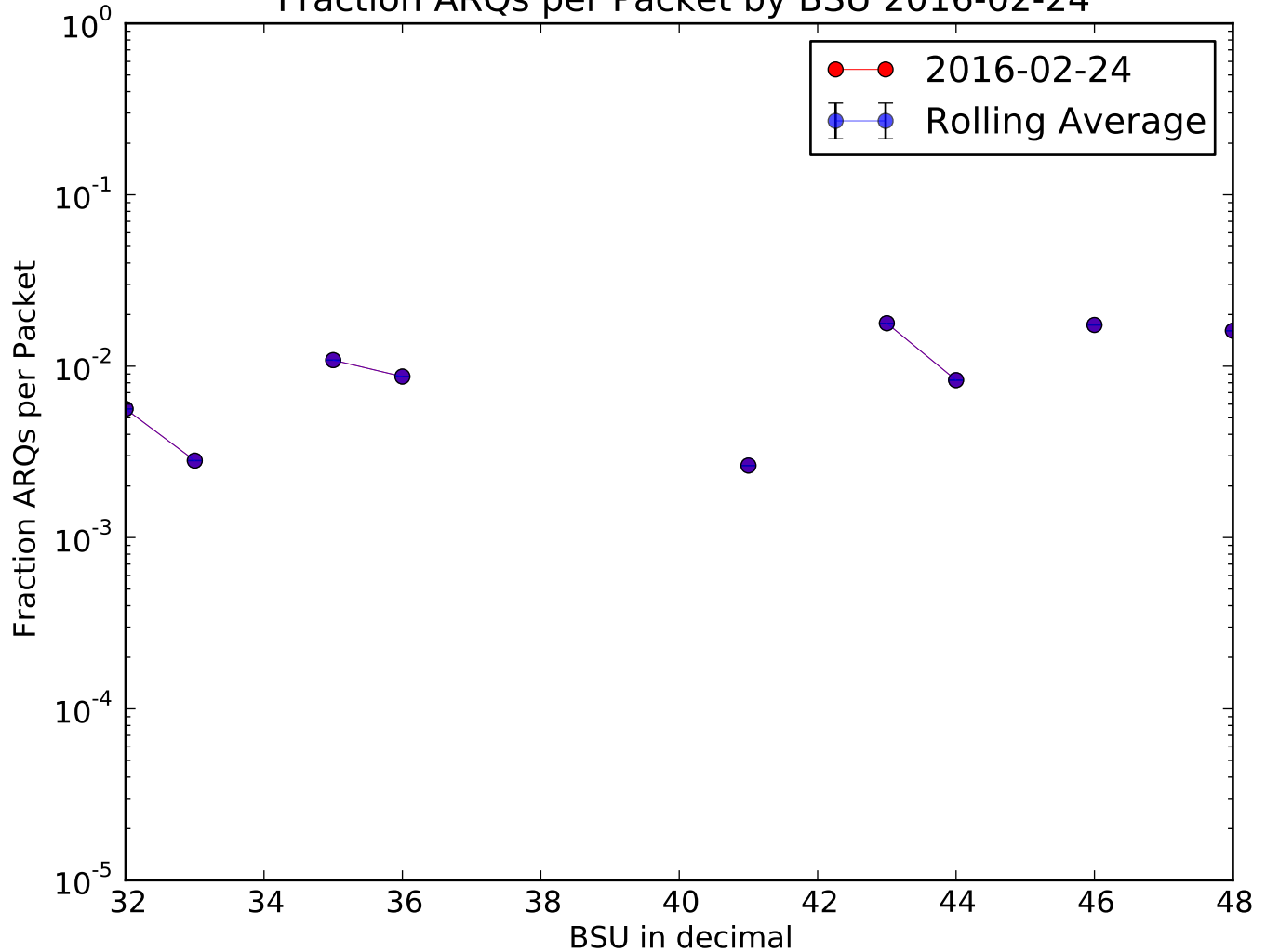
Fraction ARQs per Packet by BSU 2016-02-24
