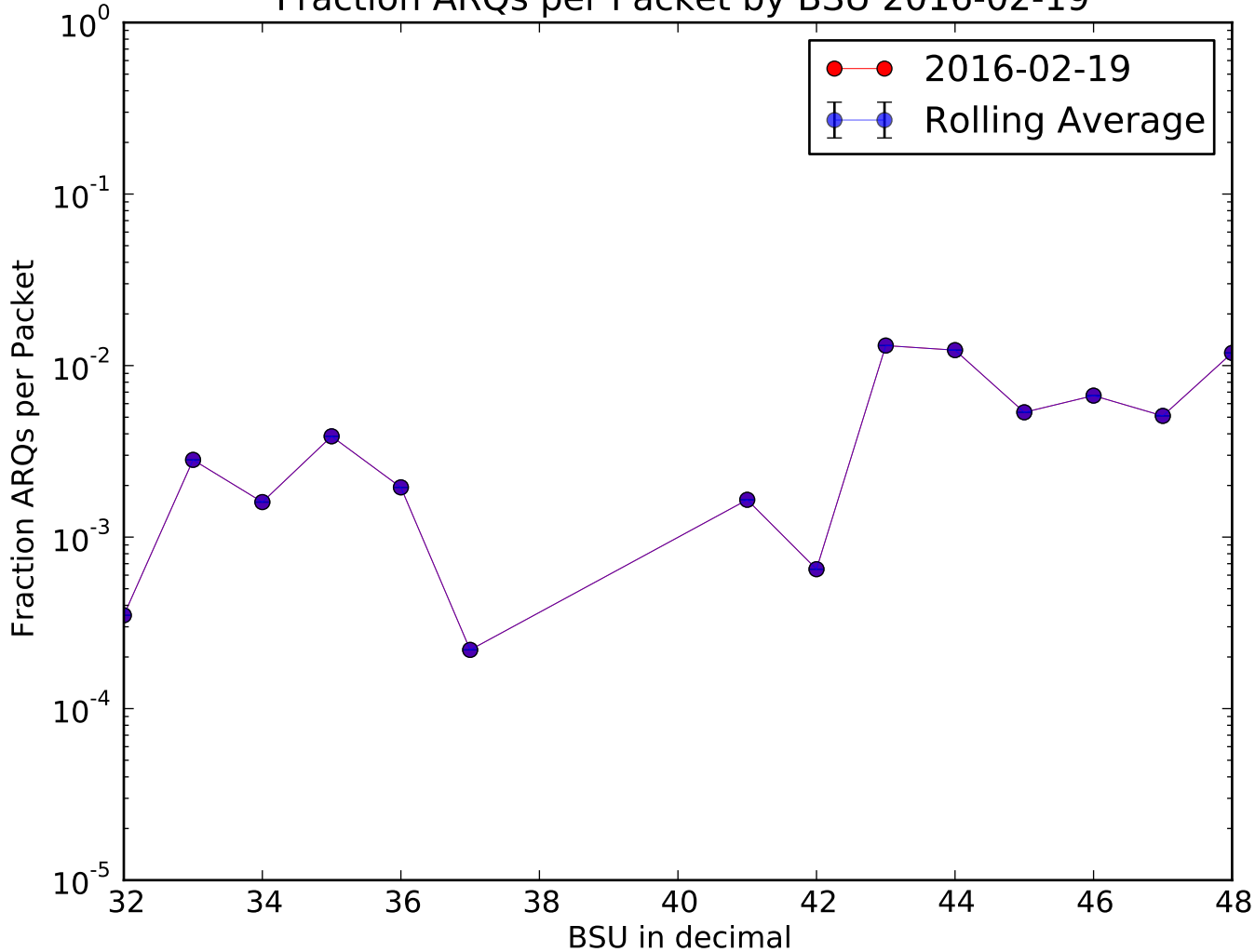
Fraction ARQs per Packet by BSU 2016-02-19
