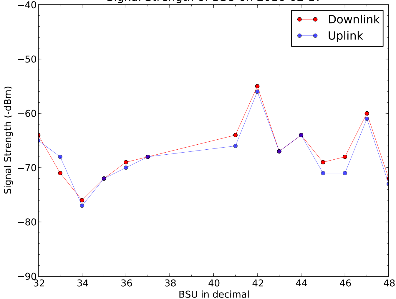
Signal Strength of BSU on 2016-02-17
