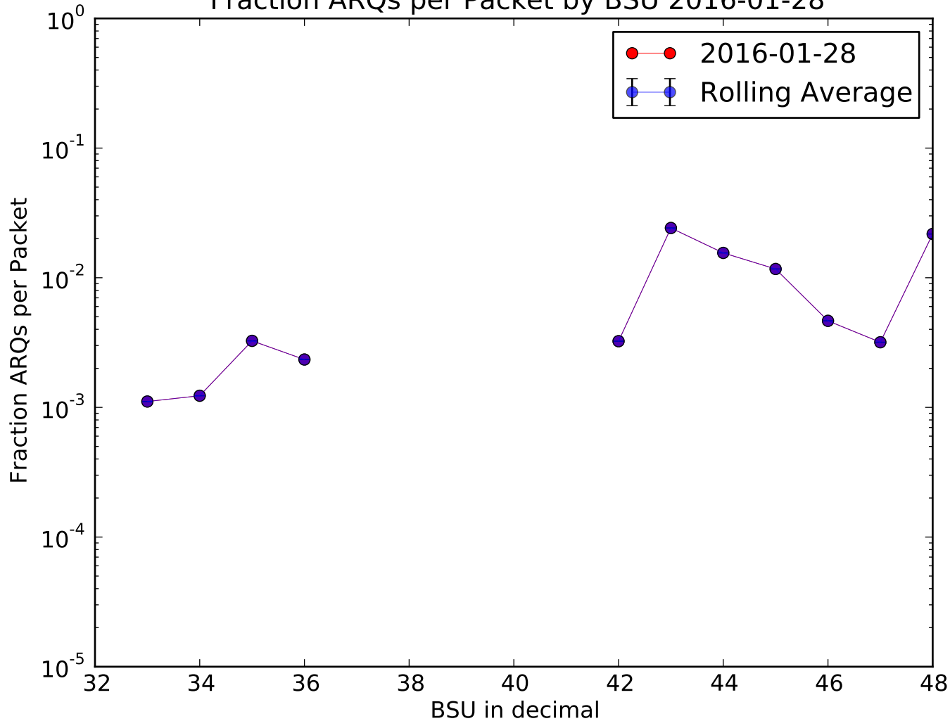
Fraction ARQs per Packet by BSU 2016-01-28
