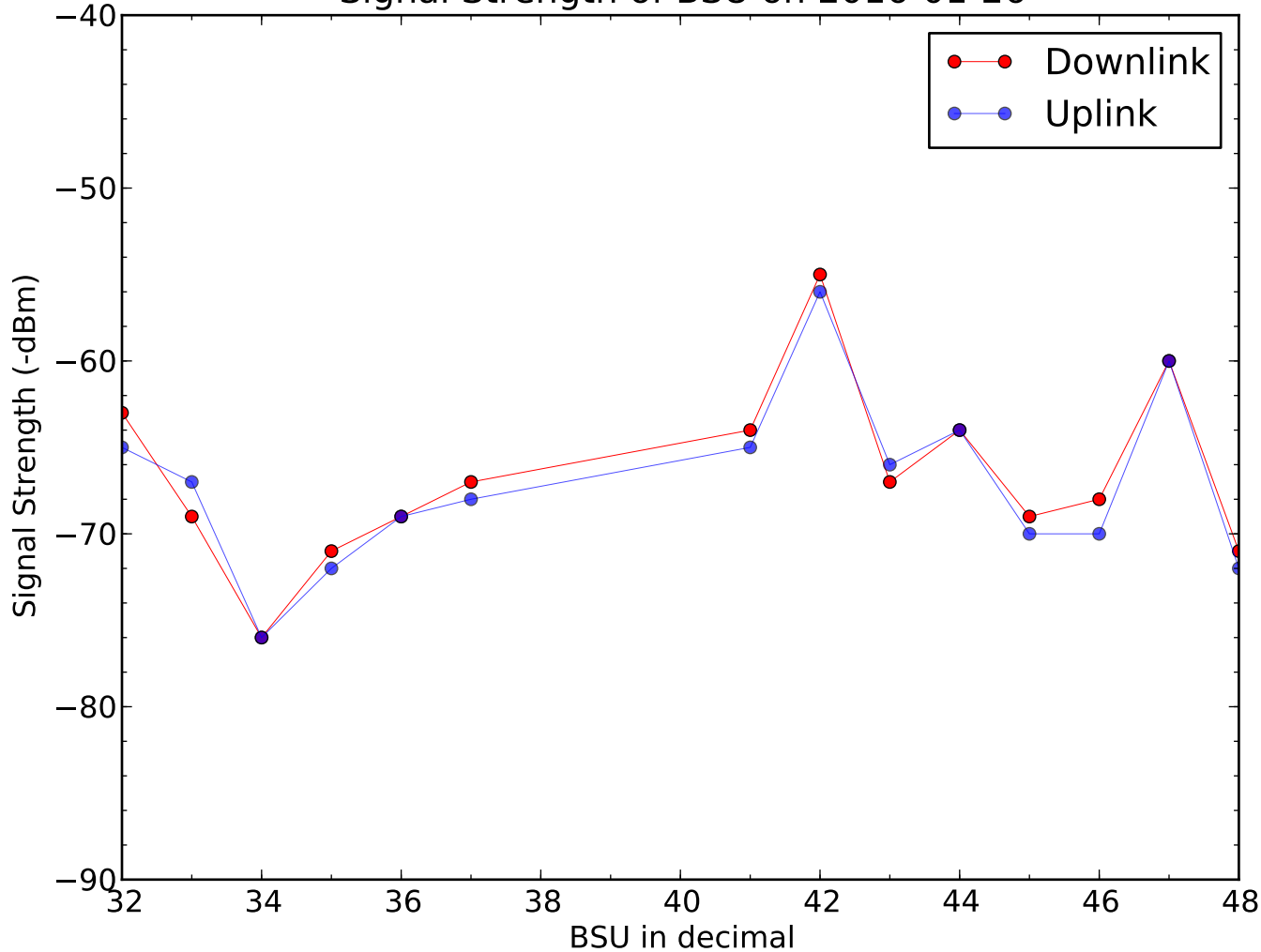
Signal Strength of BSU on 2016-01-26
