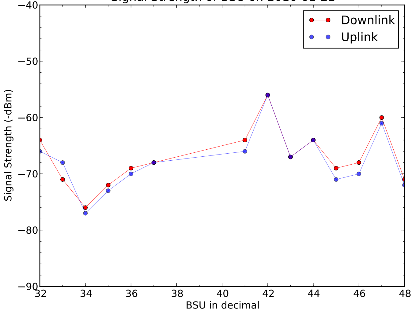
Signal Strength of BSU on 2016-01-22
