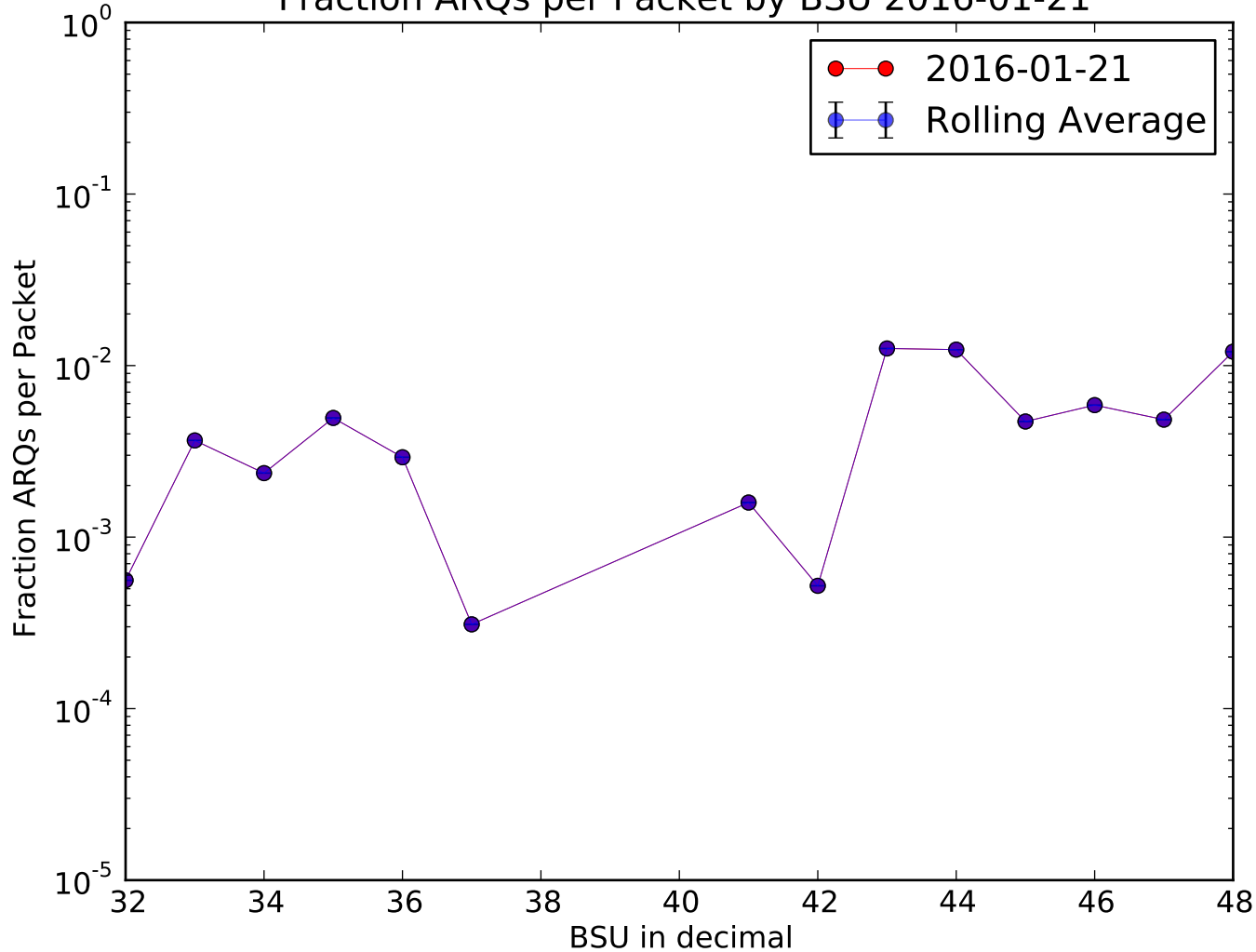
Fraction ARQs per Packet by BSU 2016-01-21
