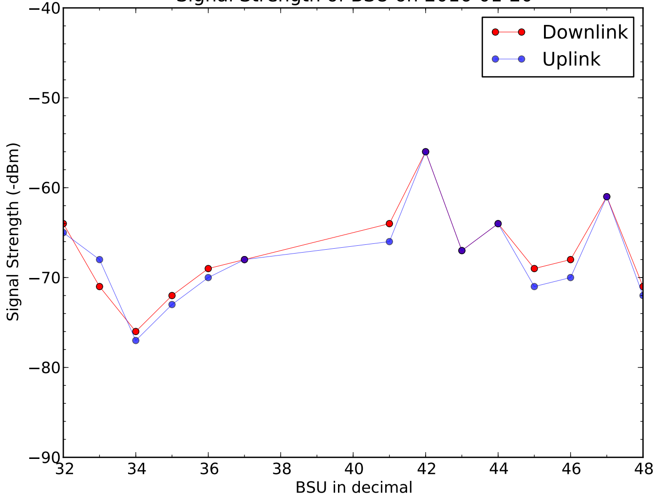
Signal Strength of BSU on 2016-01-20
