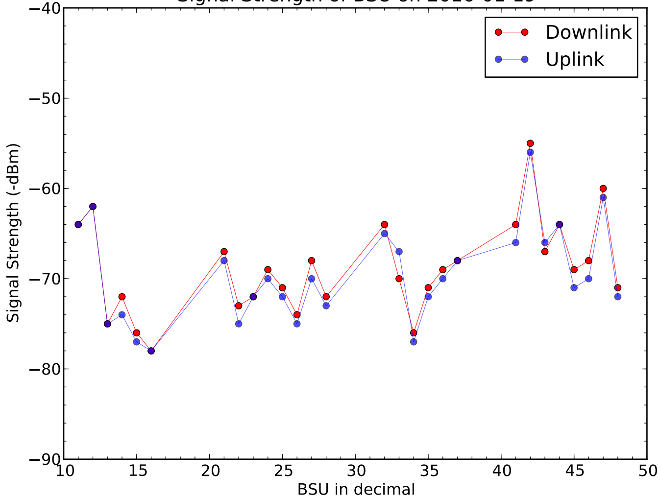
Signal Strength of BSU on 2016-01-19
