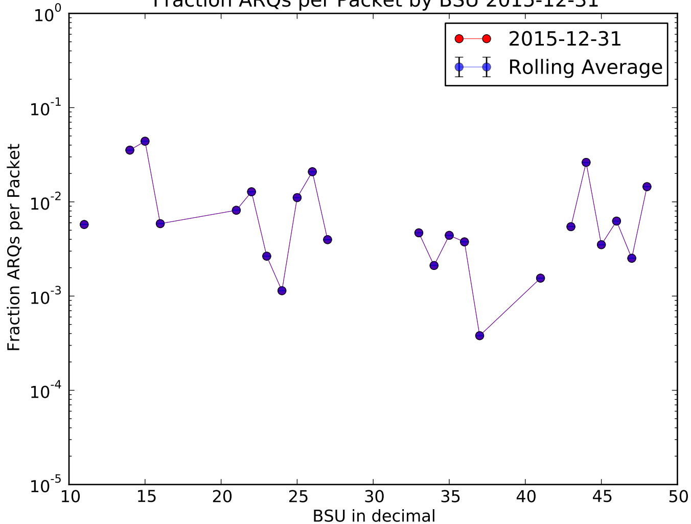
Fraction ARQs per Packet by BSU 2015-12-31
