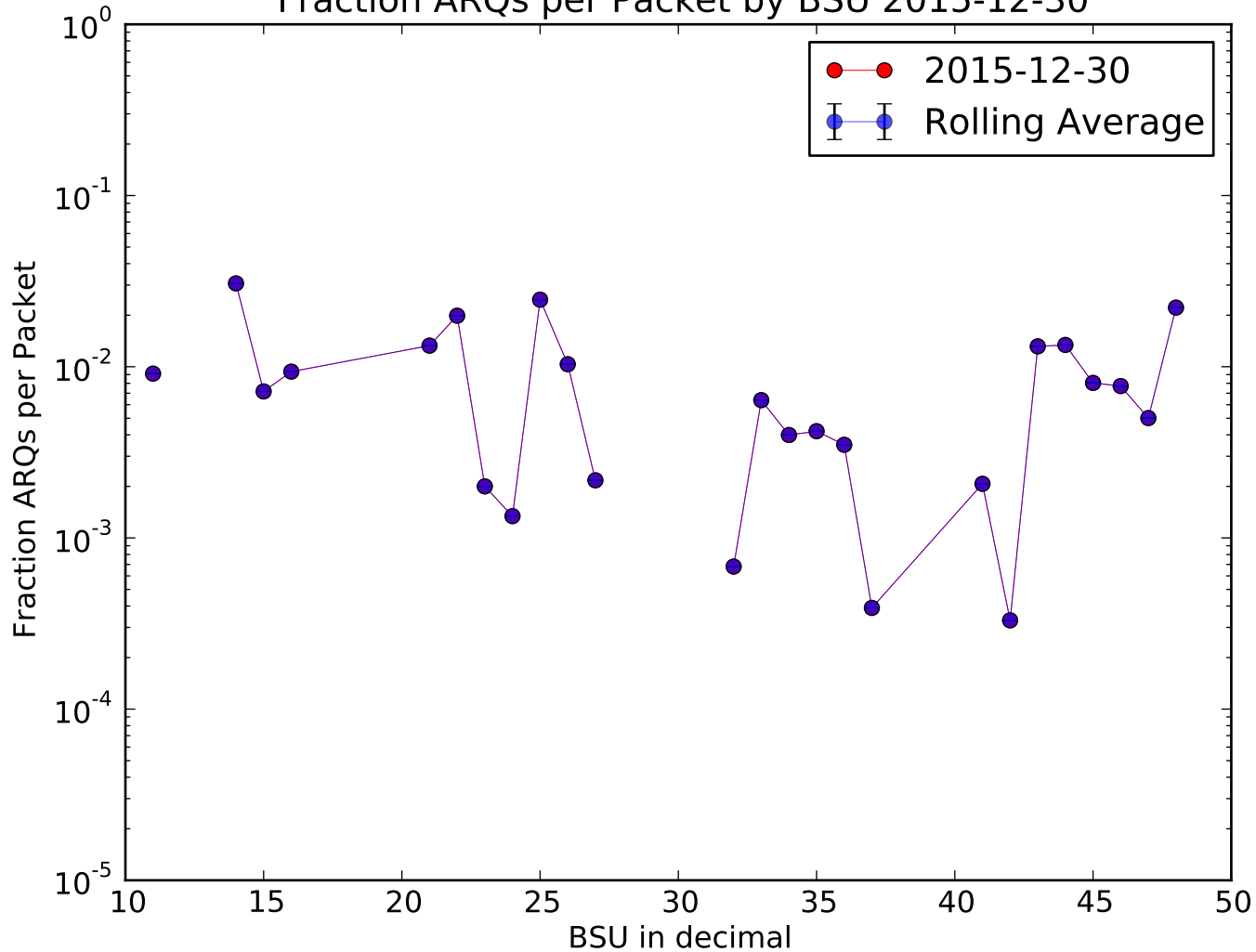
Fraction ARQs per Packet by BSU 2015-12-30
