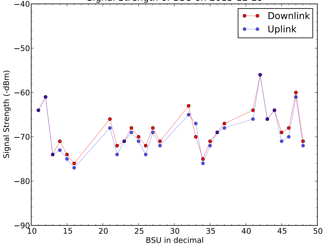
Signal Strength of BSU on 2015-12-29
