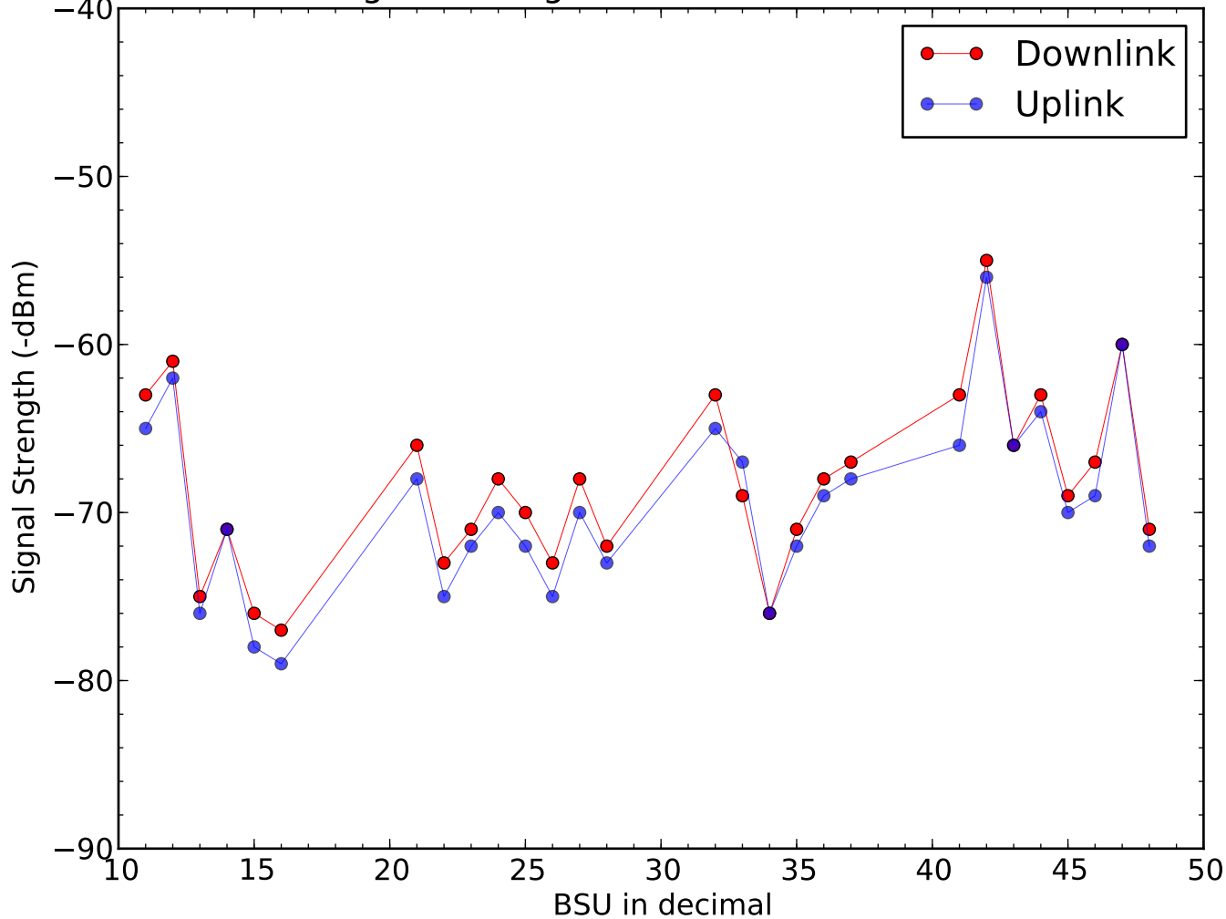
Signal Strength of BSU on 2015-12-19
