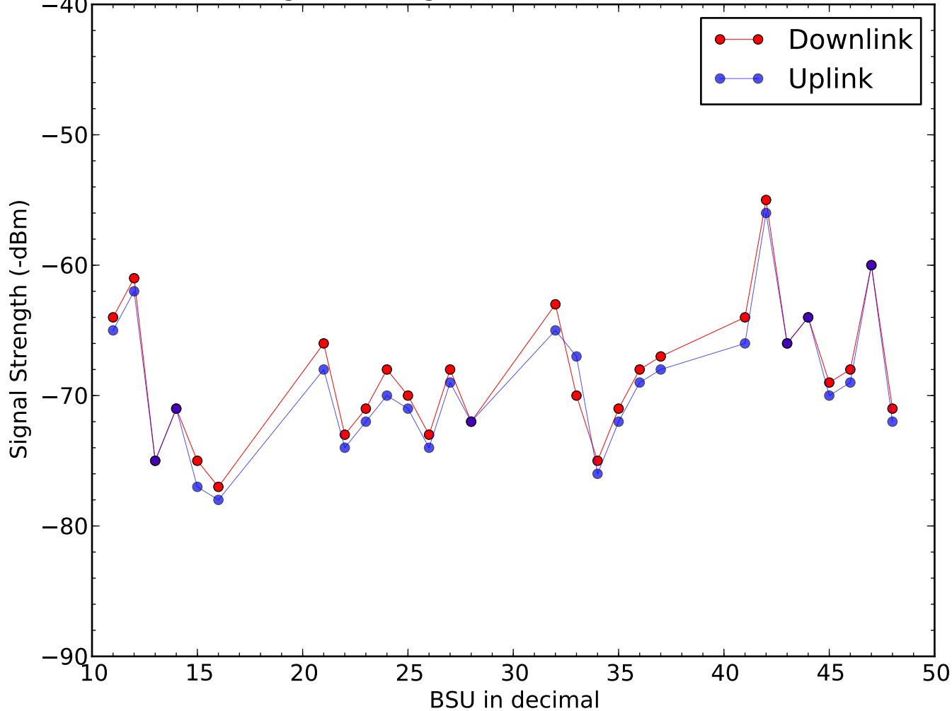
Signal Strength of BSU on 2015-12-13
