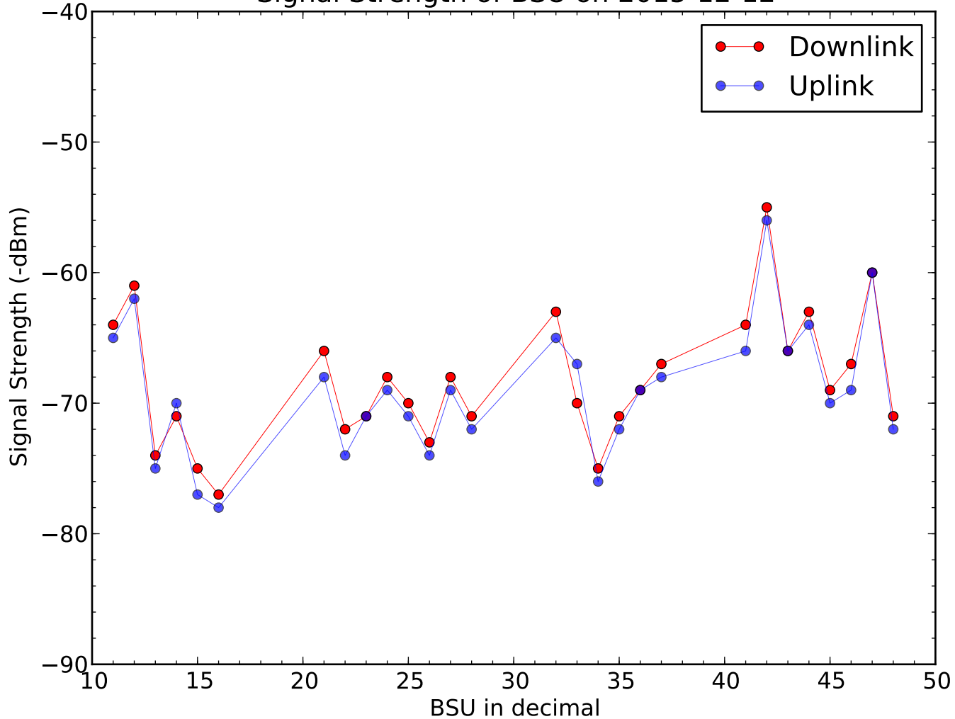
Signal Strength of BSU on 2015-12-12
