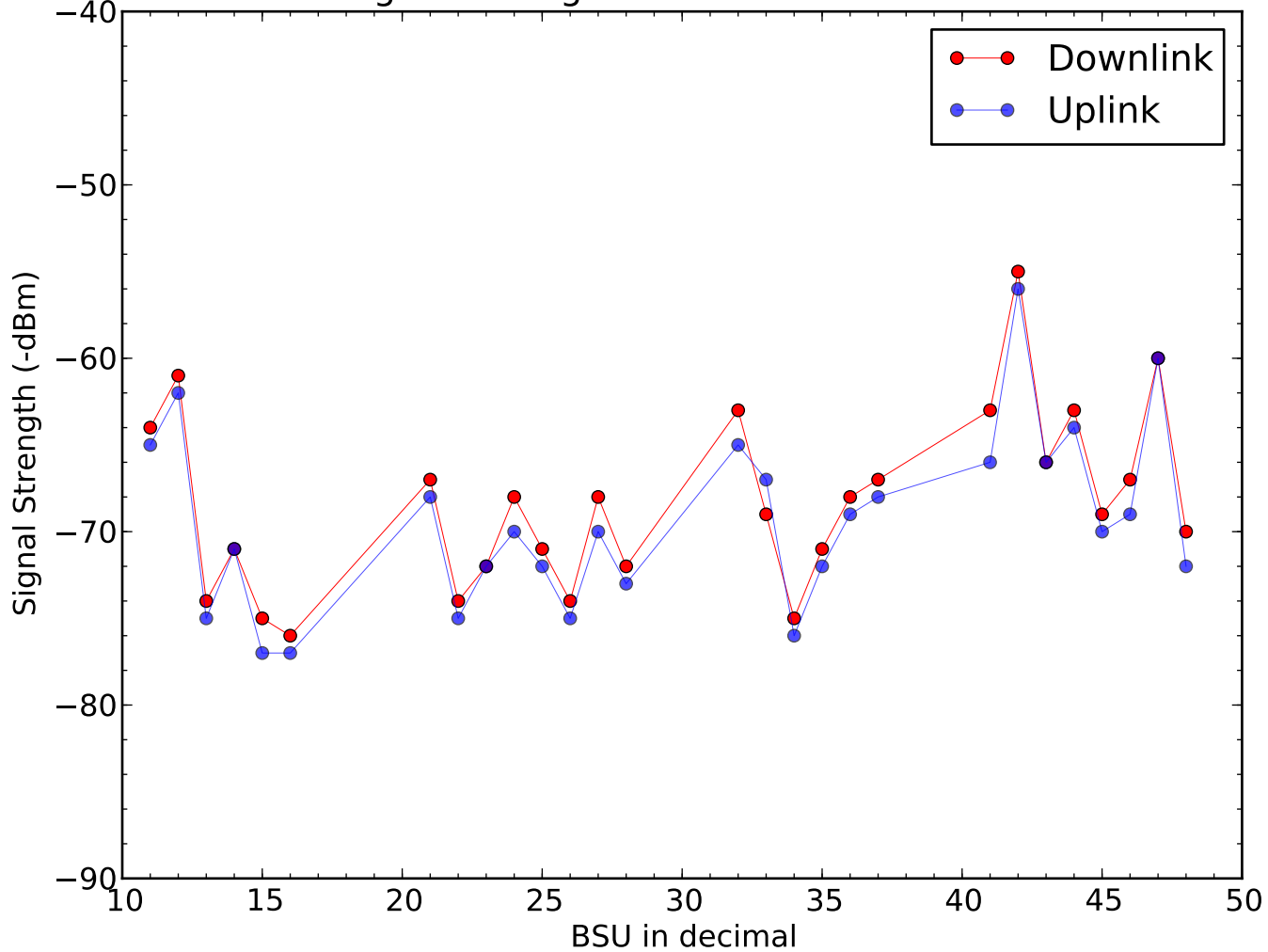
Signal Strength of BSU on 2015-12-09
