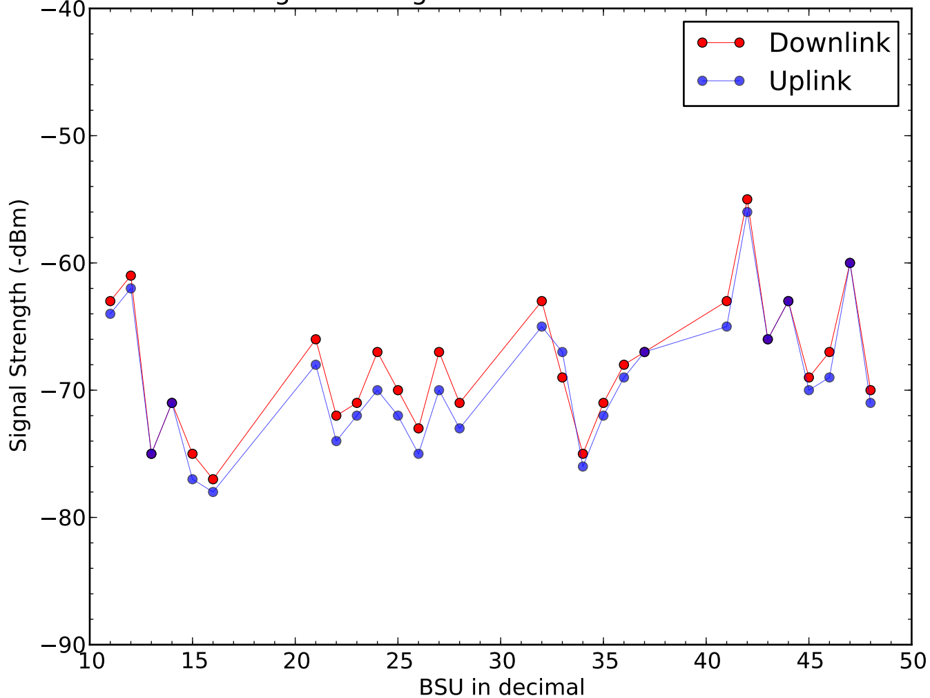
Signal Strength of BSU on 2015-11-23
