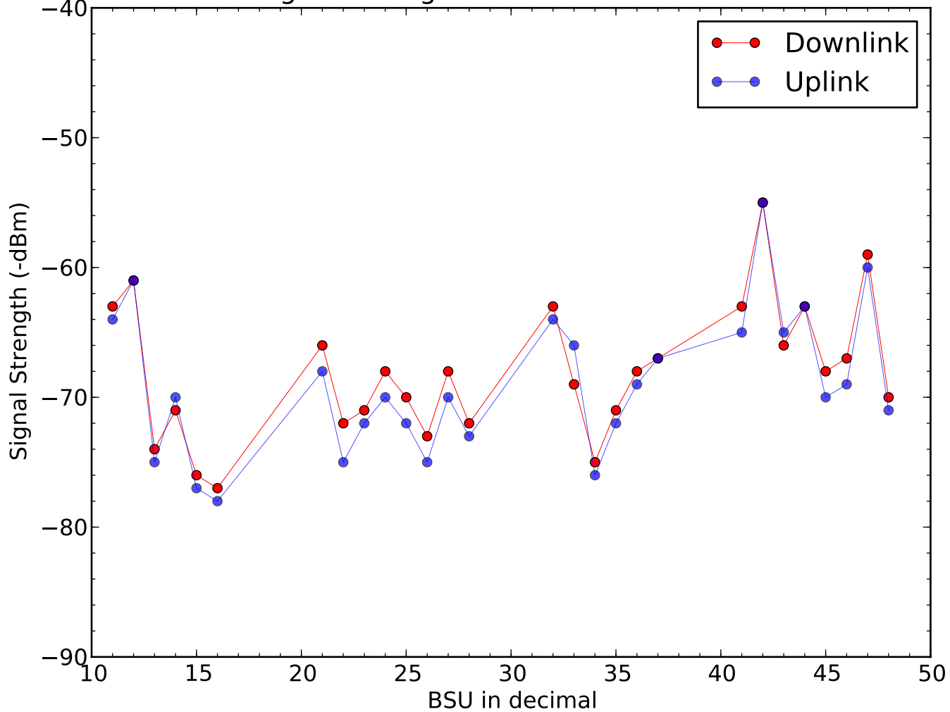
Signal Strength of BSU on 2015-11-20
