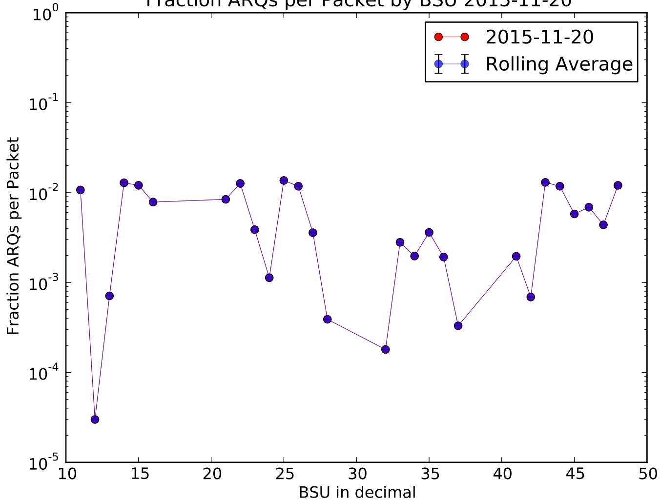
Fraction ARQs per Packet by BSU 2015-11-20
