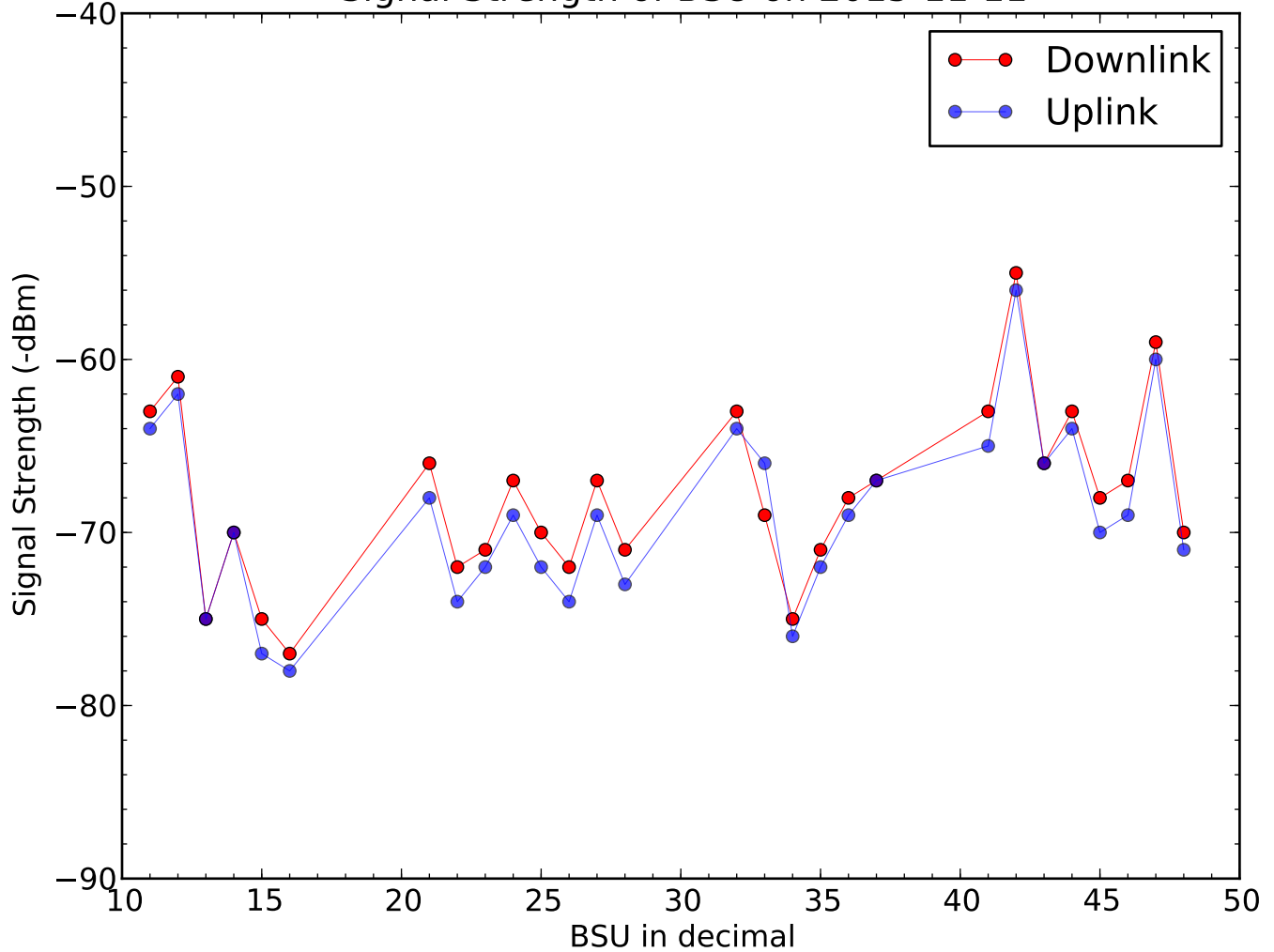
Signal Strength of BSU on 2015-11-11
