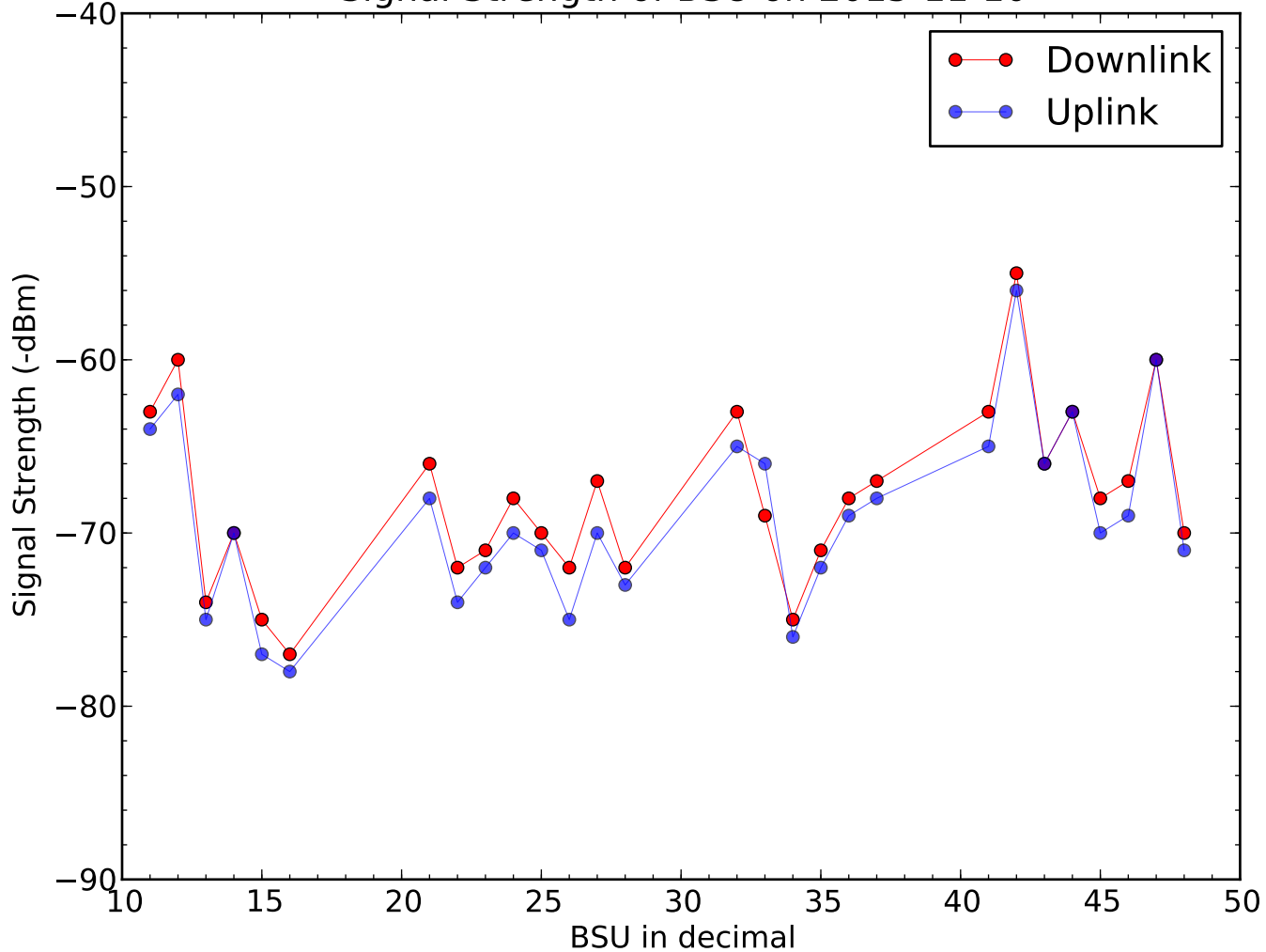
Signal Strength of BSU on 2015-11-10
