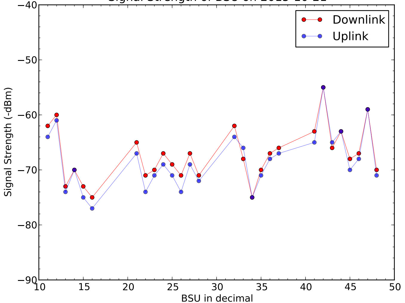
Signal Strength of BSU on 2015-10-21
