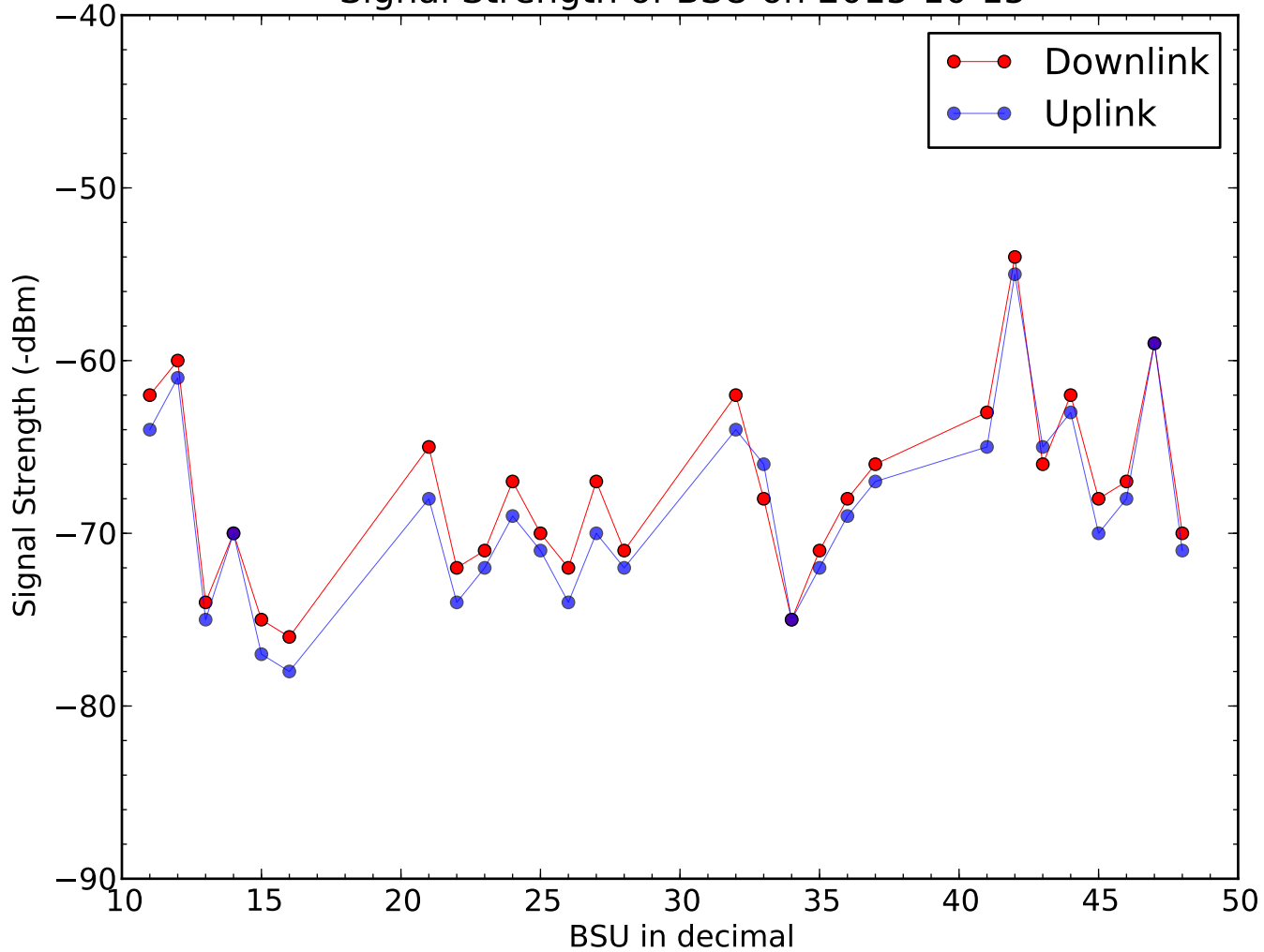
Signal Strength of BSU on 2015-10-15
