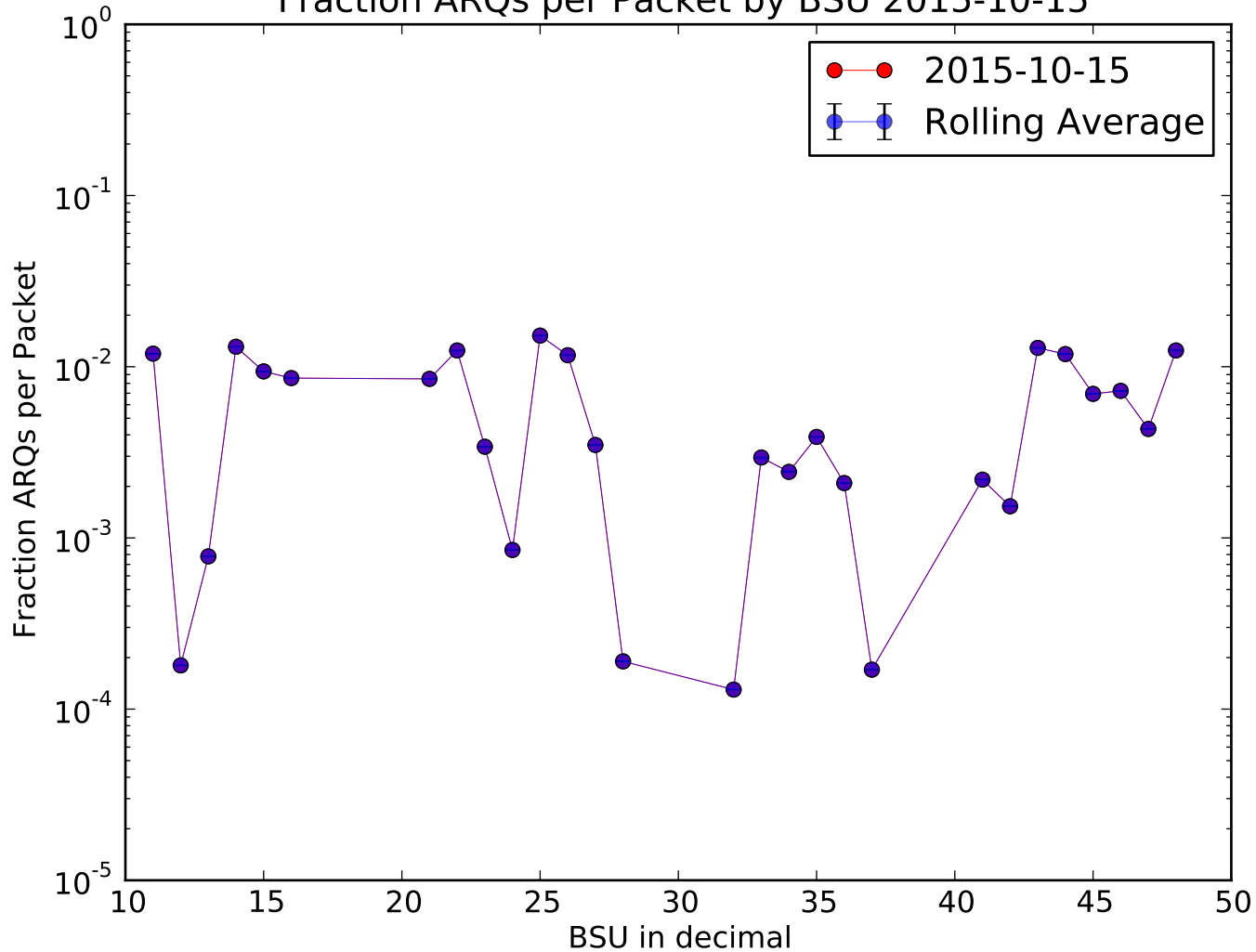
Fraction ARQs per Packet by BSU 2015-10-15
