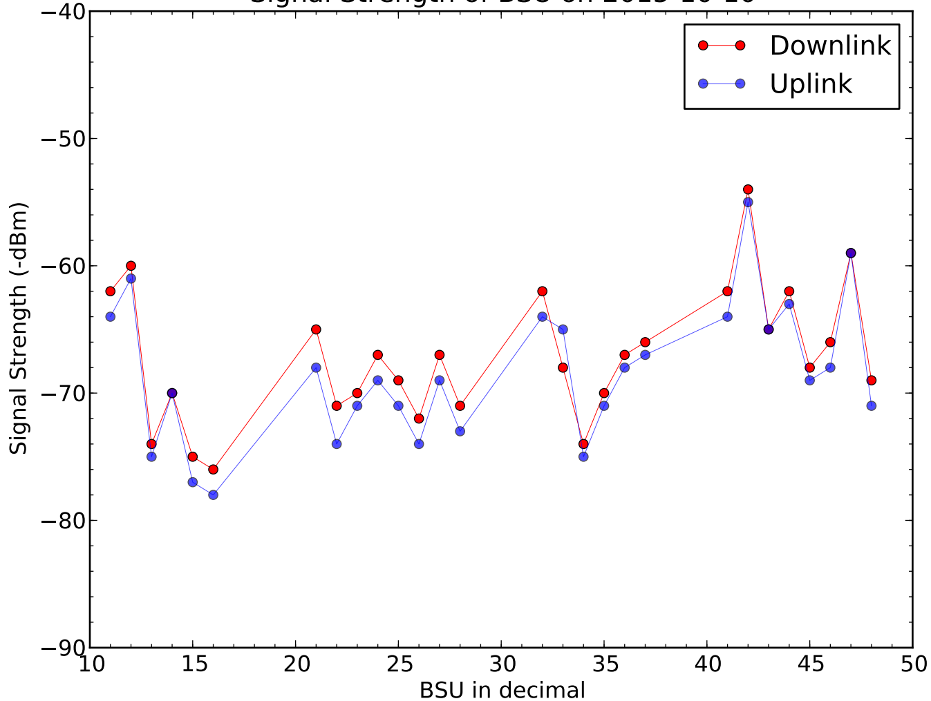
Signal Strength of BSU on 2015-10-10
