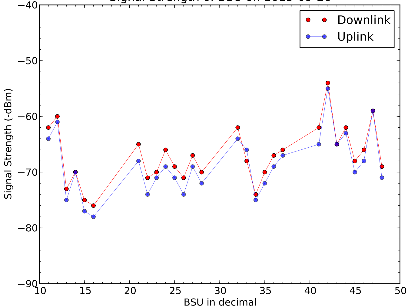
Signal Strength of BSU on 2015-09-26
