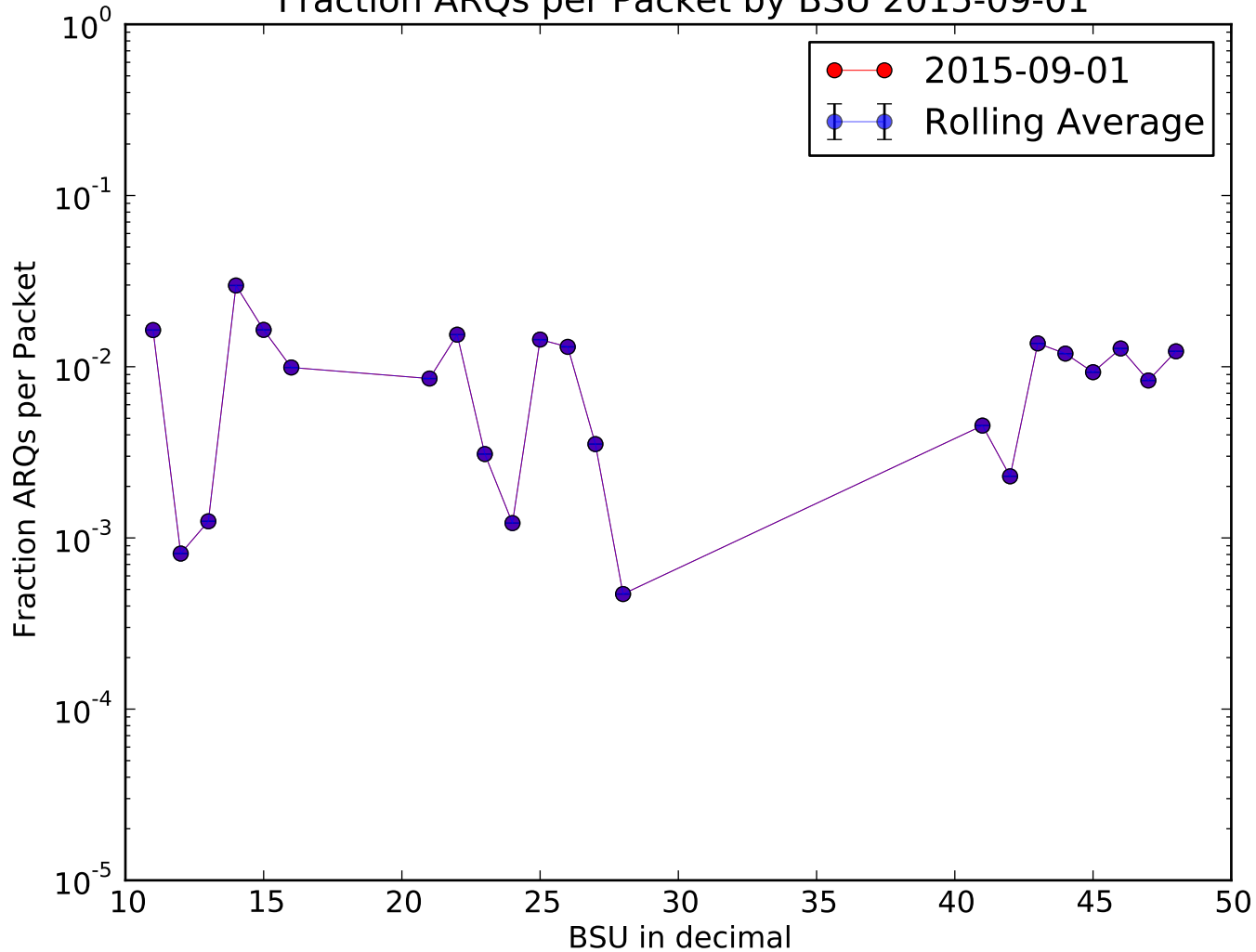
Fraction ARQs per Packet by BSU 2015-09-01
