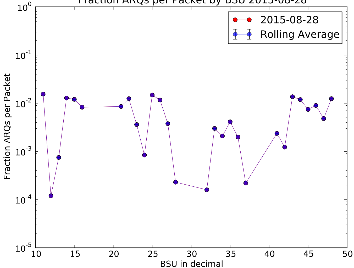
Fraction ARQs per Packet by BSU 2015-08-28
