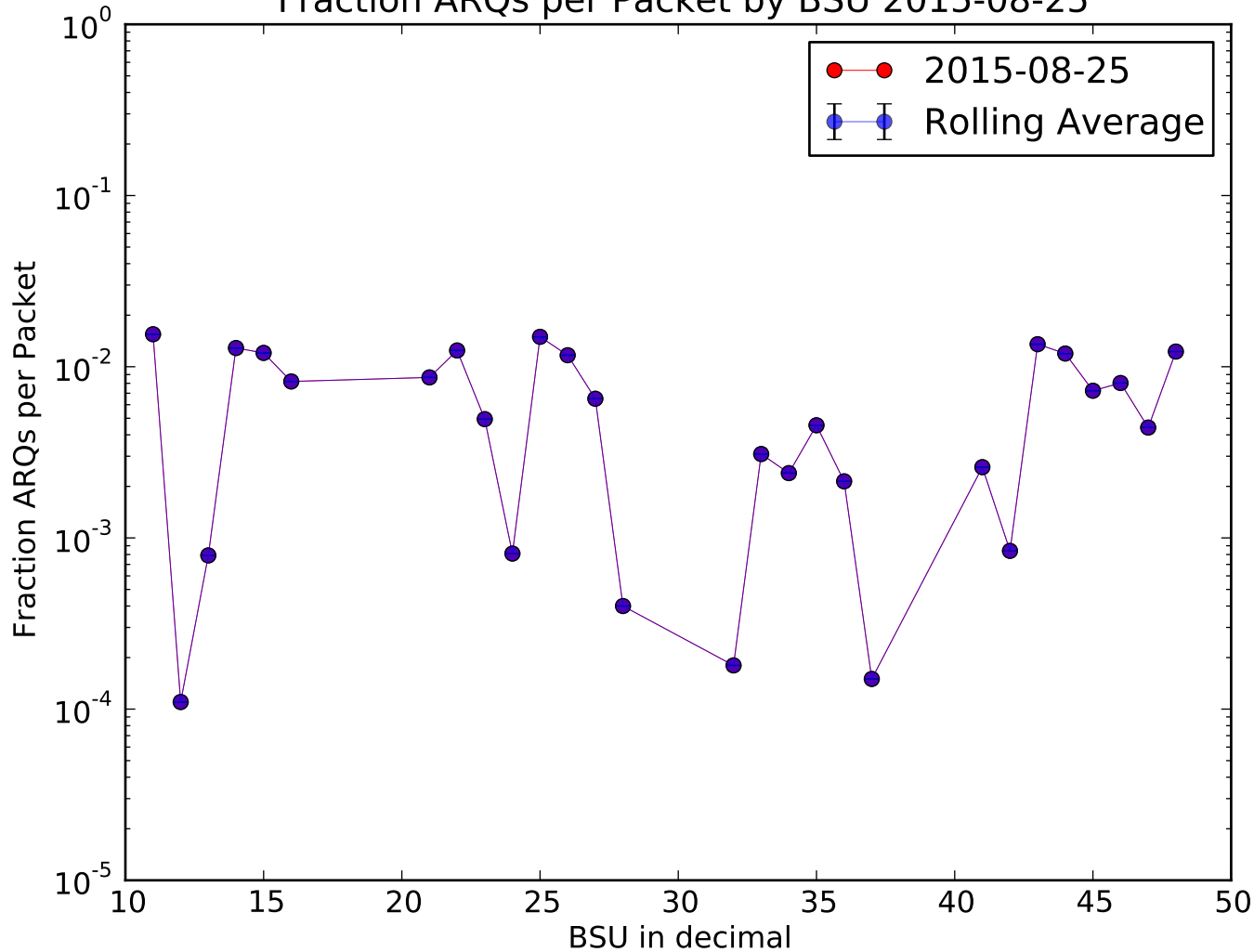
Fraction ARQs per Packet by BSU 2015-08-25
