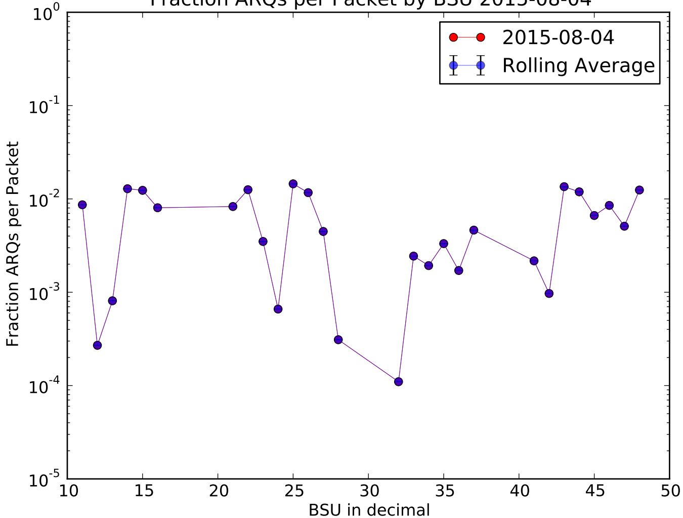
Fraction ARQs per Packet by BSU 2015-08-04
