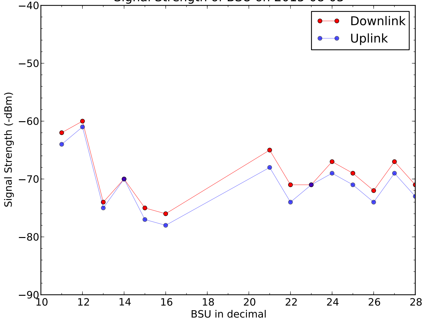
Signal Strength of BSU on 2015-08-03
