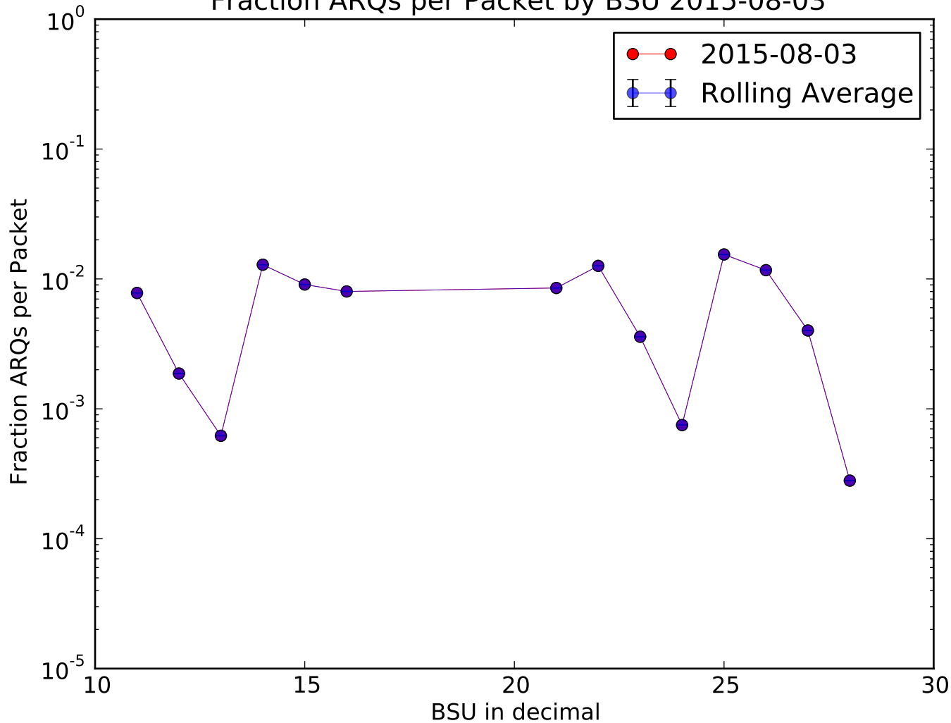
Fraction ARQs per Packet by BSU 2015-08-03
