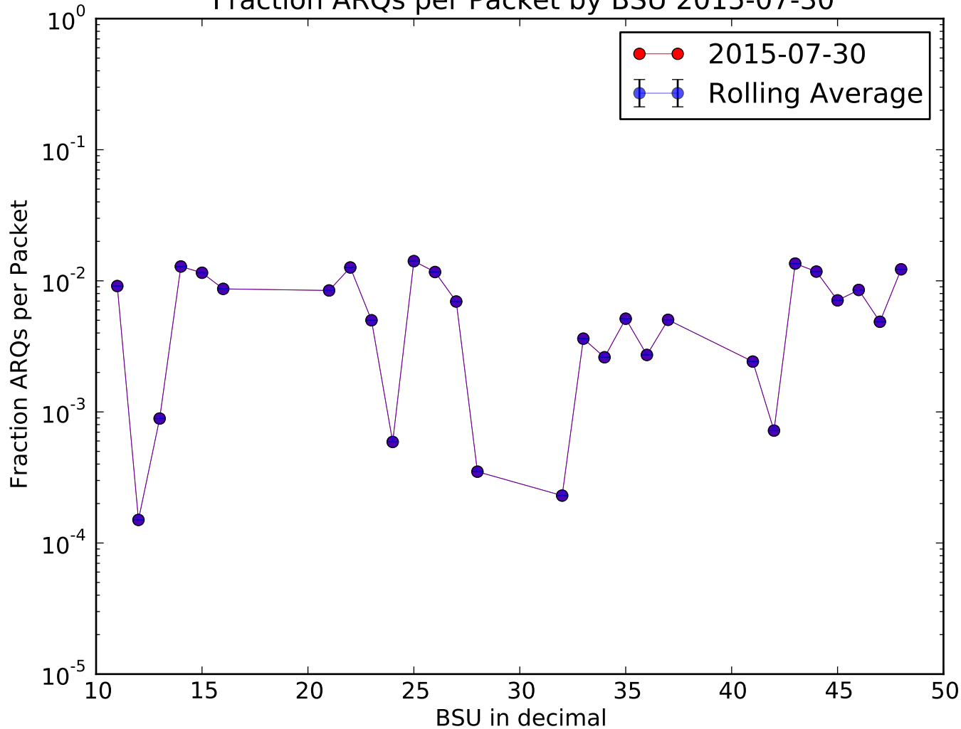
Fraction ARQs per Packet by BSU 2015-07-30
