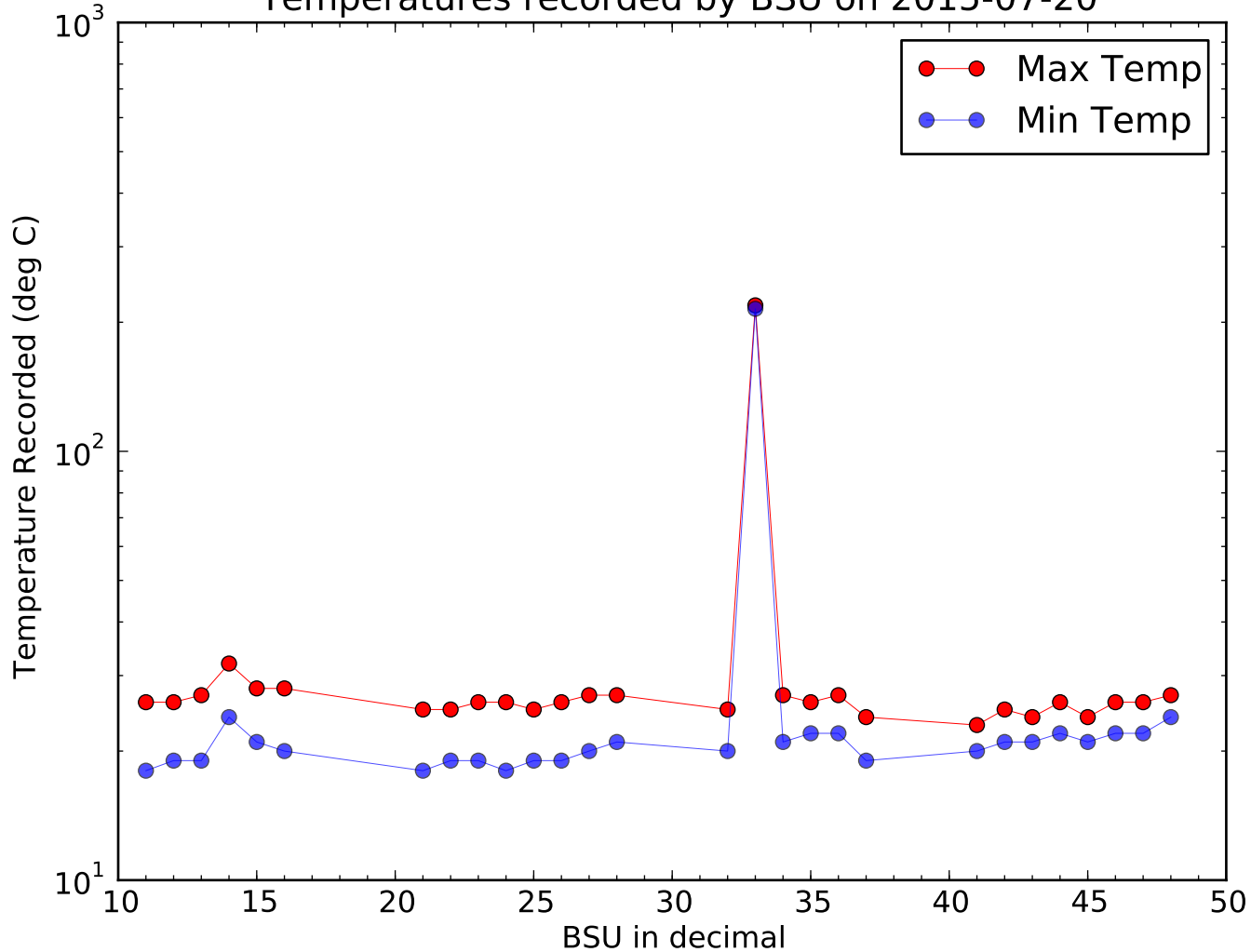
Temperatures recorded by BSU on 2015-07-20
