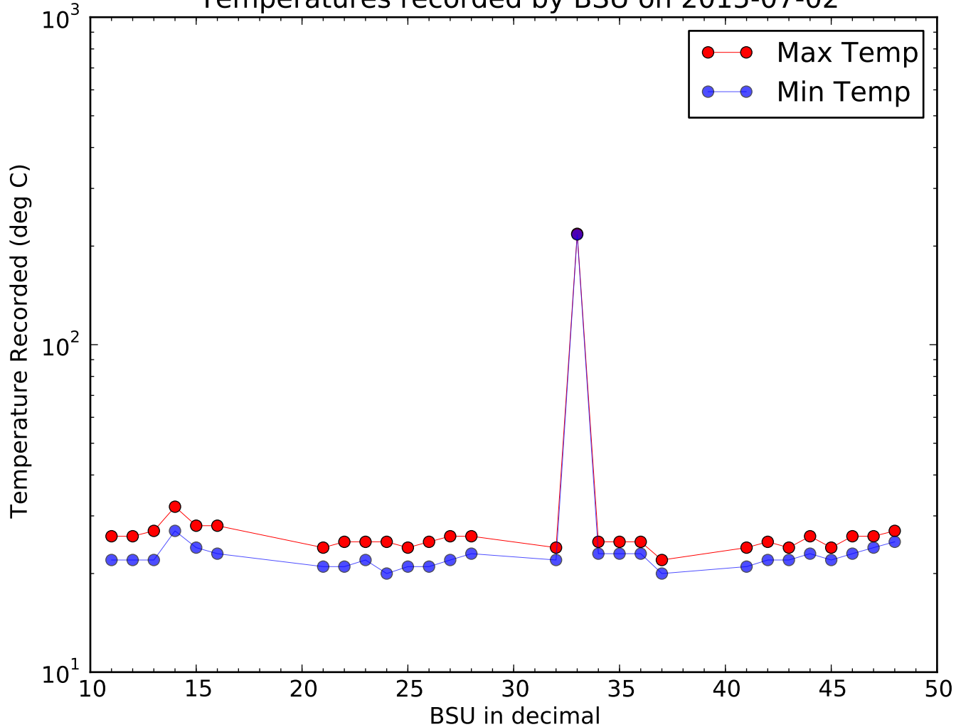
Temperatures recorded by BSU on 2015-07-02
