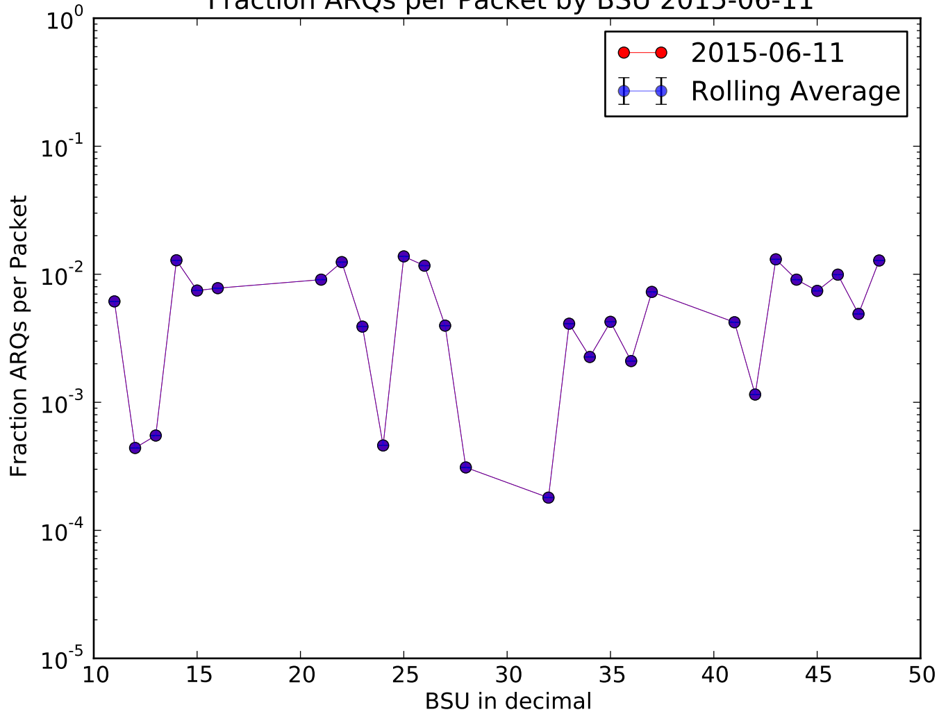
Fraction ARQs per Packet by BSU 2015-06-11
