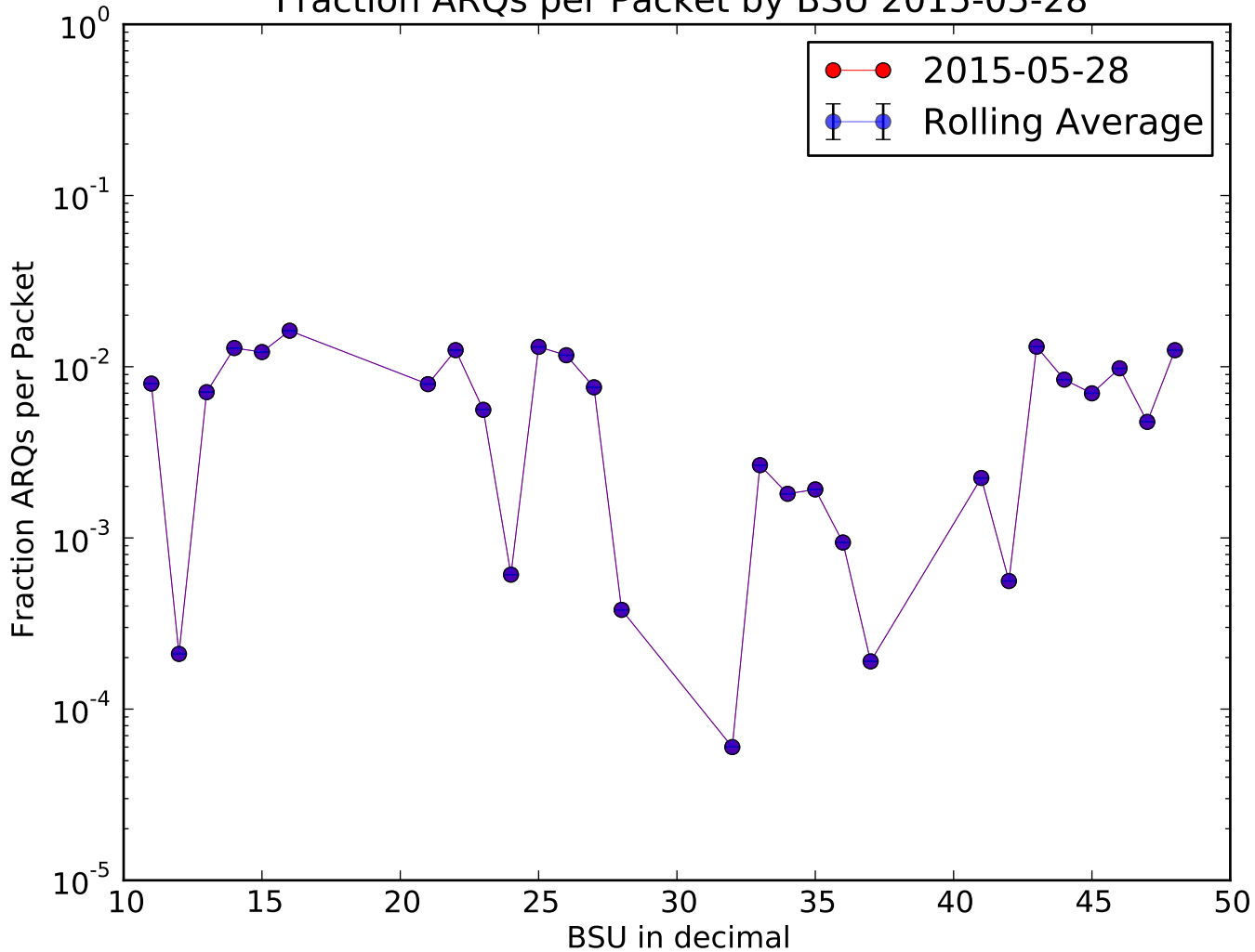
Fraction ARQs per Packet by BSU 2015-05-28
