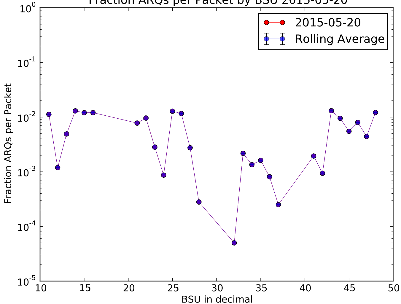
Fraction ARQs per Packet by BSU 2015-05-20
