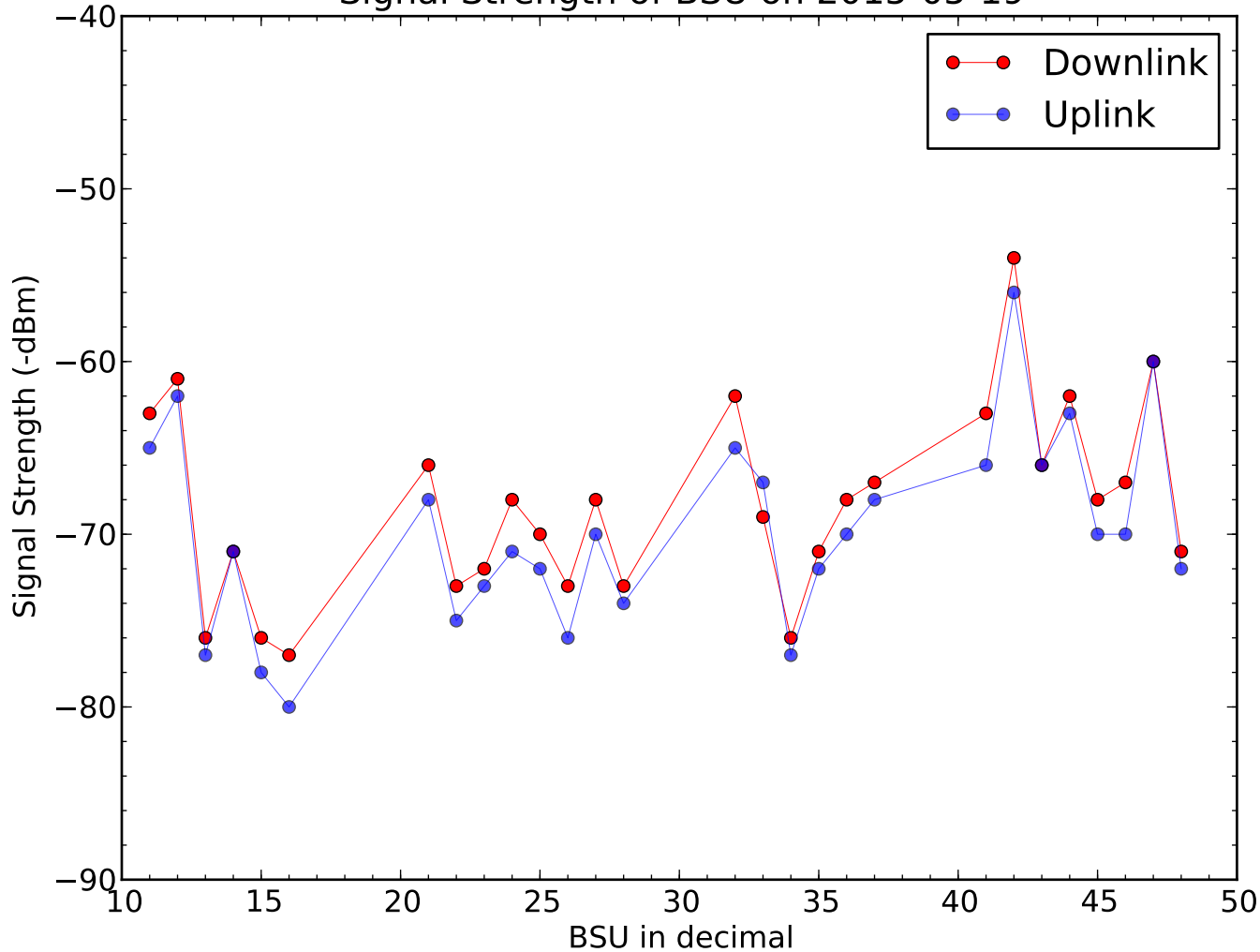
Signal Strength of BSU on 2015-05-19
